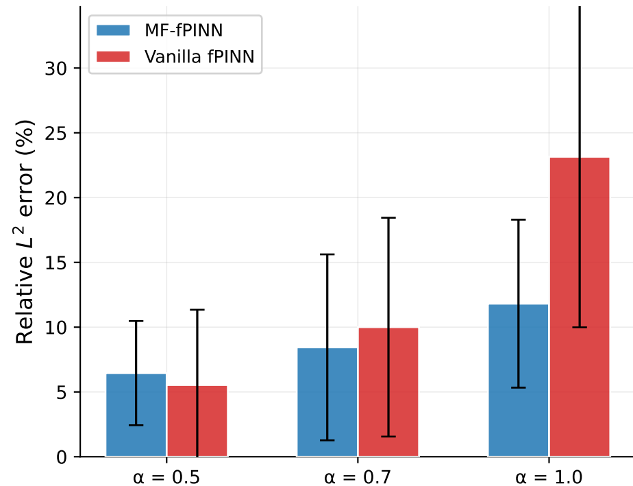
(a) MF-fPINN vs Vanilla at N_{\text{col}} = 100
