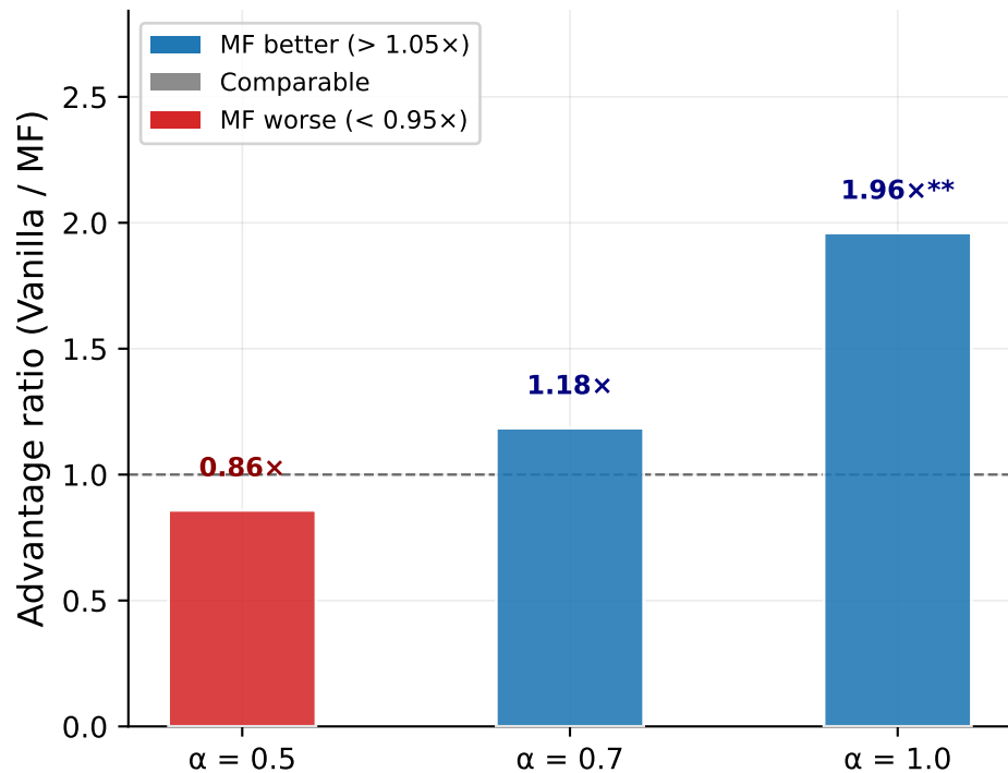
(b) MF advantage factor ( N_{\text{terms}} = 12 , 10 seeds)
