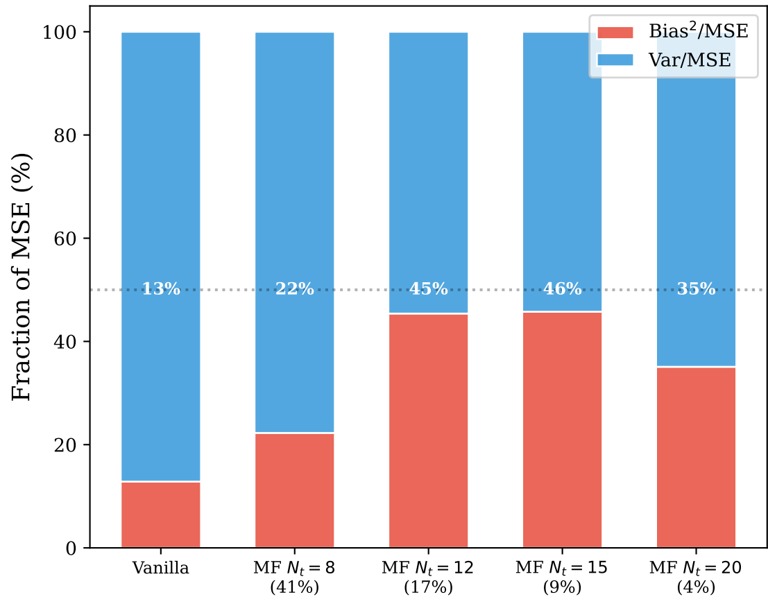
(b) Bias vs variance dominance
