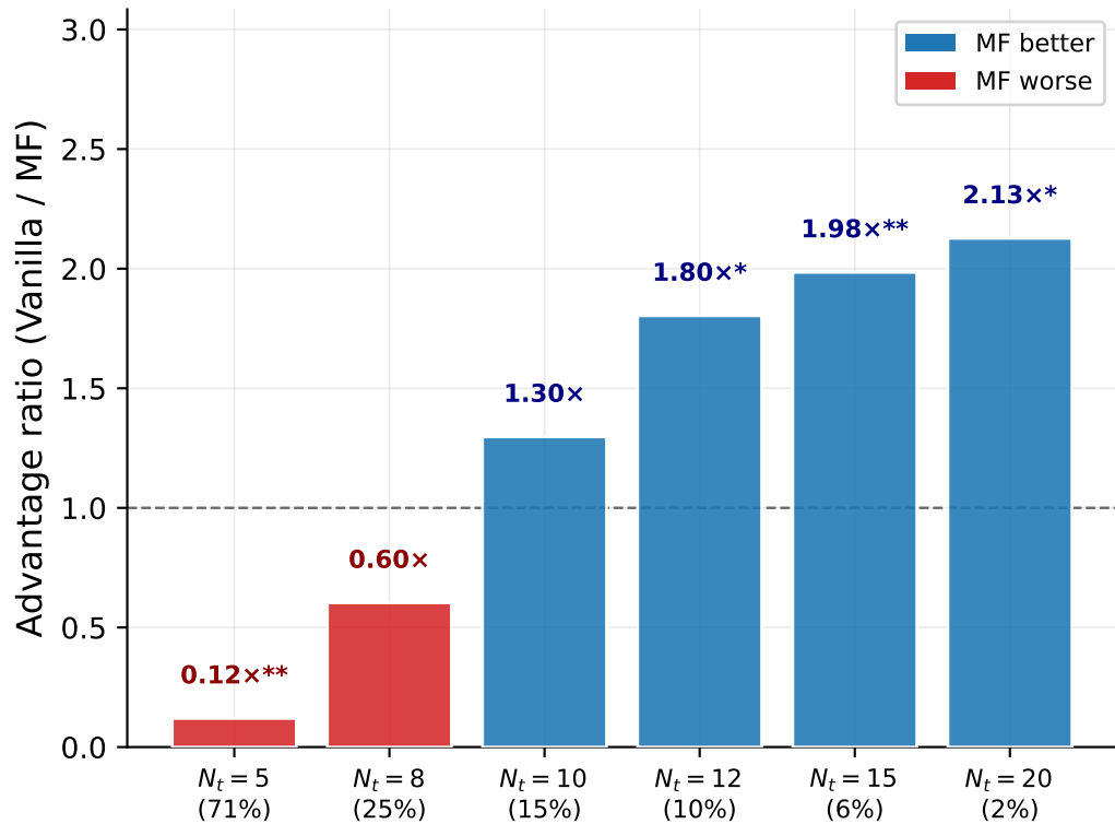
(b) Monotonic advantage at \alpha = 1.0
