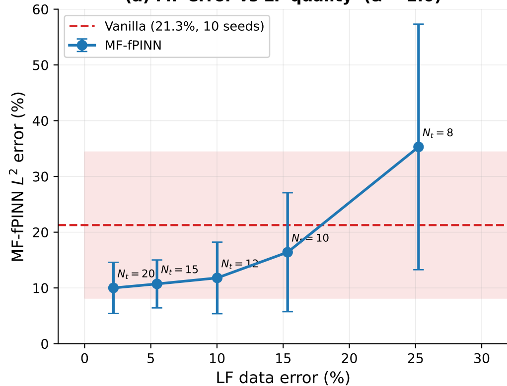
(a) MF error vs LF quality ( \alpha = 1.0 )
