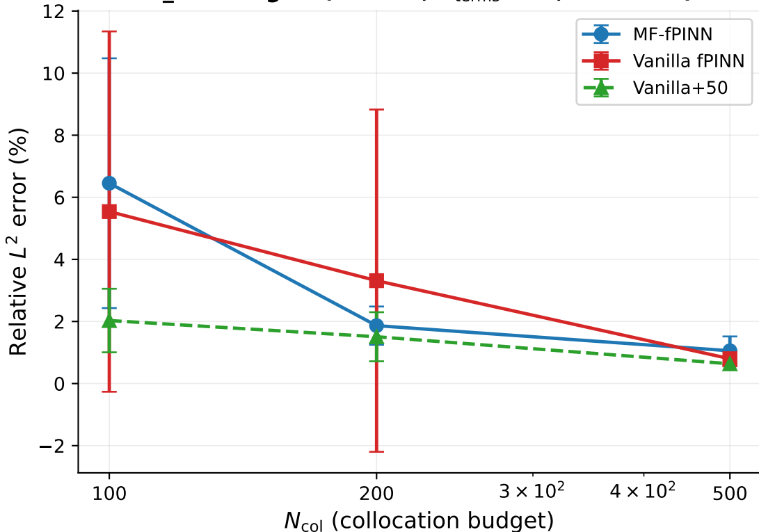
N_col budget ( \alpha = 0.5 , N_{\text{terms}} = 12 , 10 seeds)
