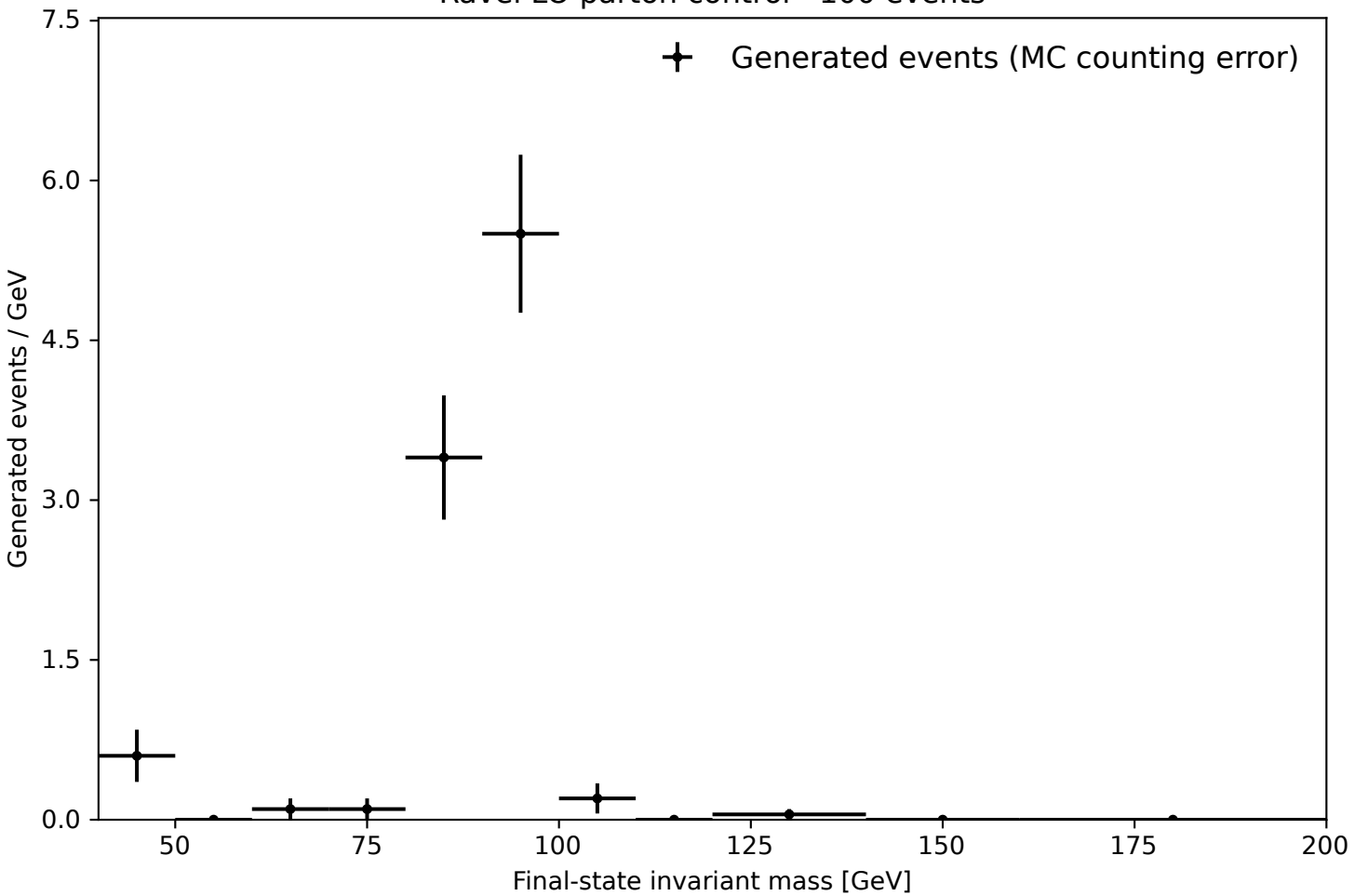
Ravel LO parton control · 100 events
