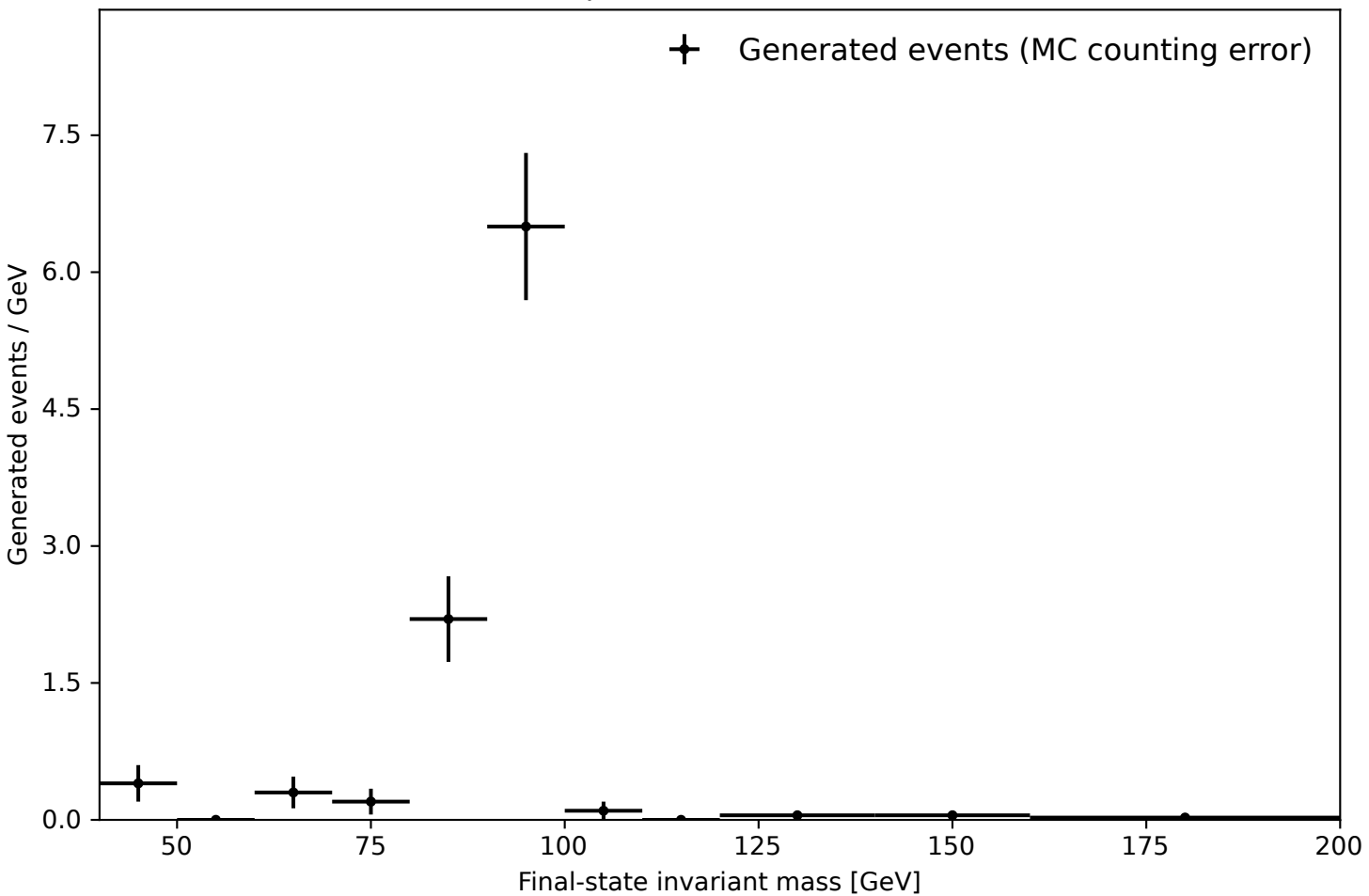
Ravel LO parton control · 100 events
