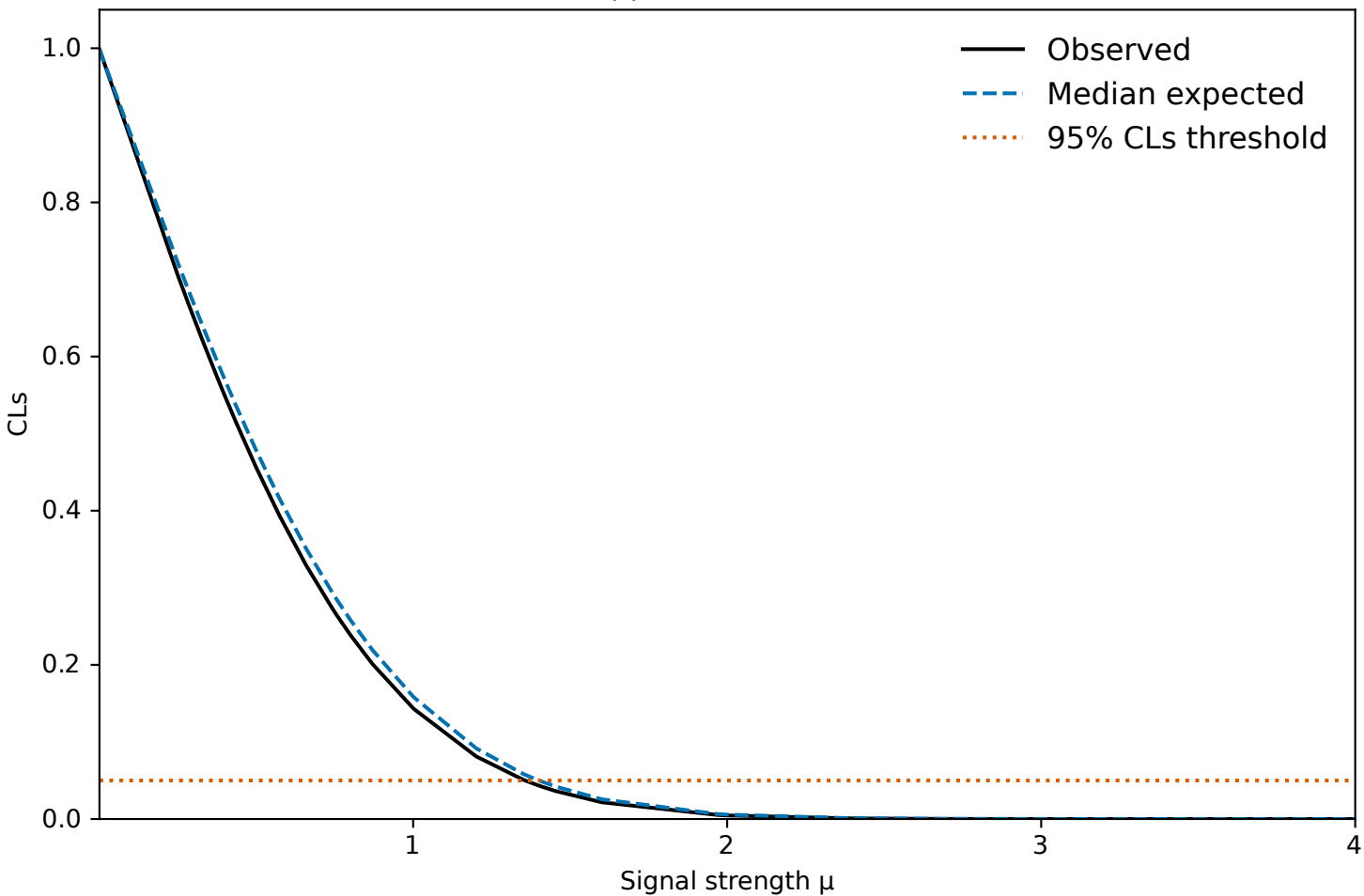
Ravel supplied-likelihood control
