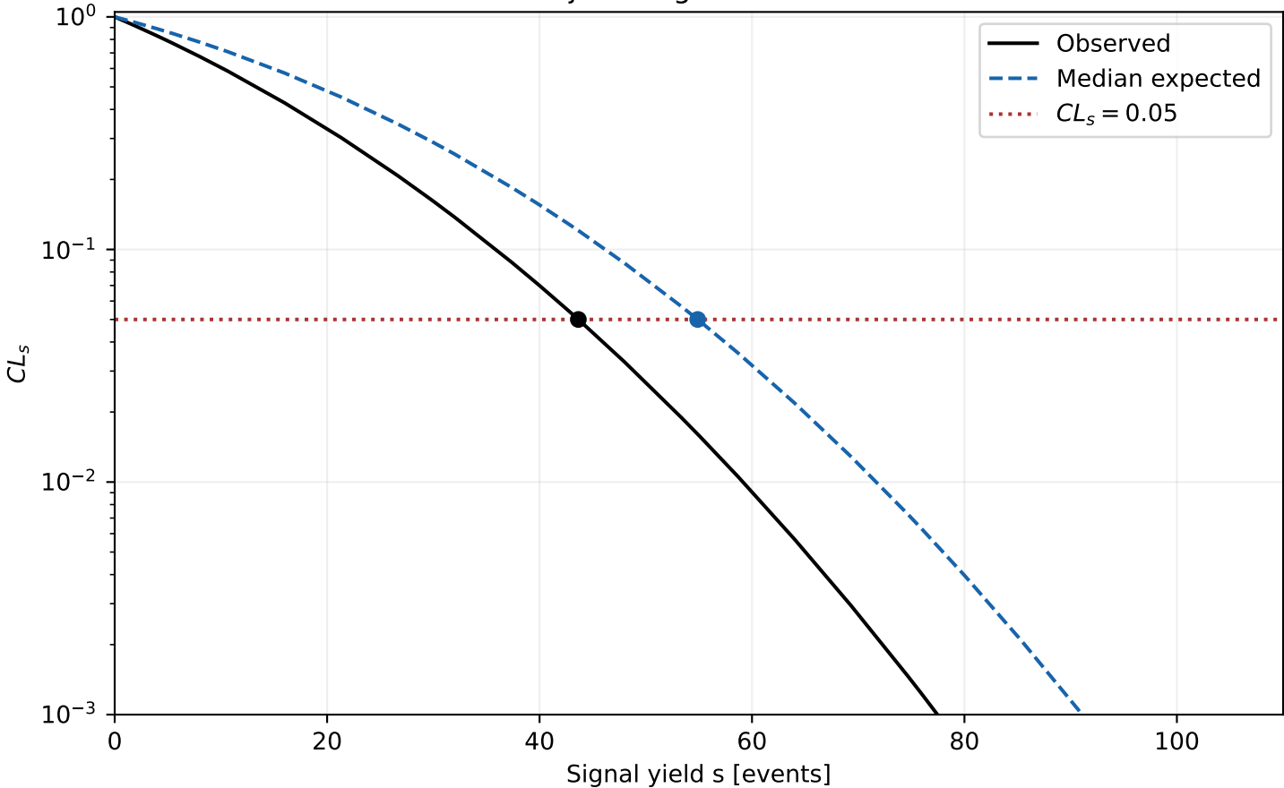
ATLAS 2016 2jl — single-bin statistical control
