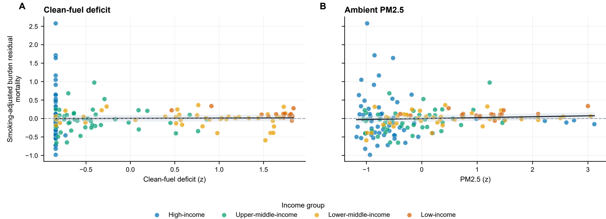
Figure S8. Smoking-adjusted burden residual scatter diagnostics
