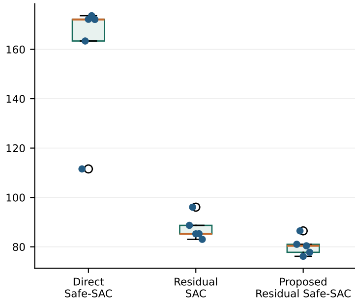
Tracking RMSE (kW)
