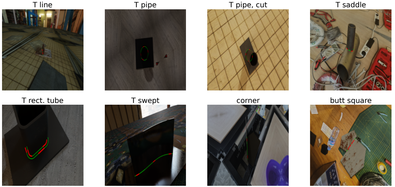
Fig. 2. Tier 2: rendered views of the same benchmark (one per stratum, view 0 = the tier-1 camera), with the constructed seam (green) and tack (red) masks. Not used in the results below.
