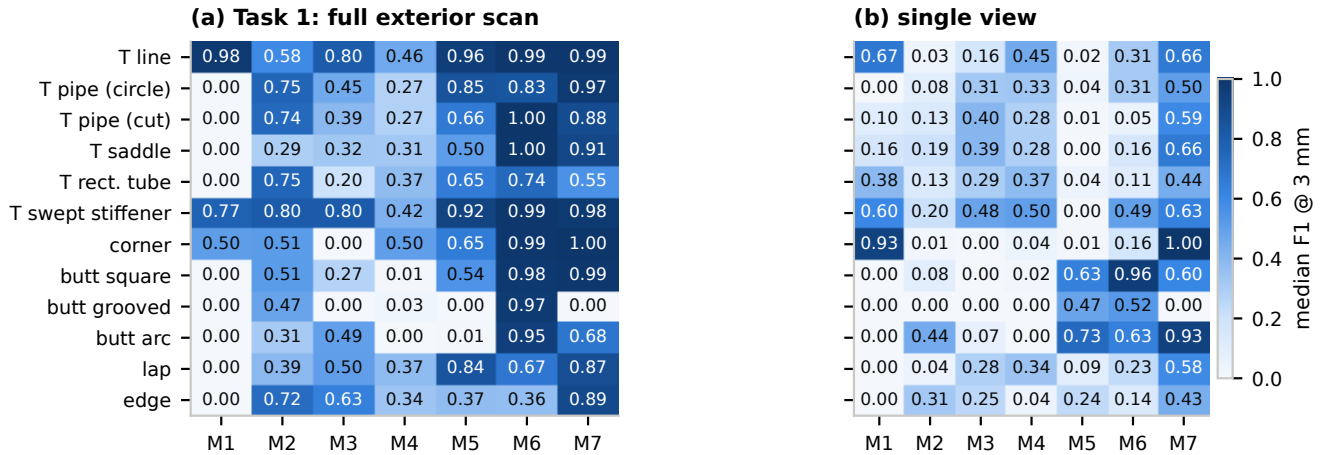
Fig. 3. Median F1 at 3 mm per stratum and method: (a) Task 1, every weldable seam from a perfect exterior scan; (b) the same methods on what one camera returns. M6 is given the model of every scene and has no L1 arm.
