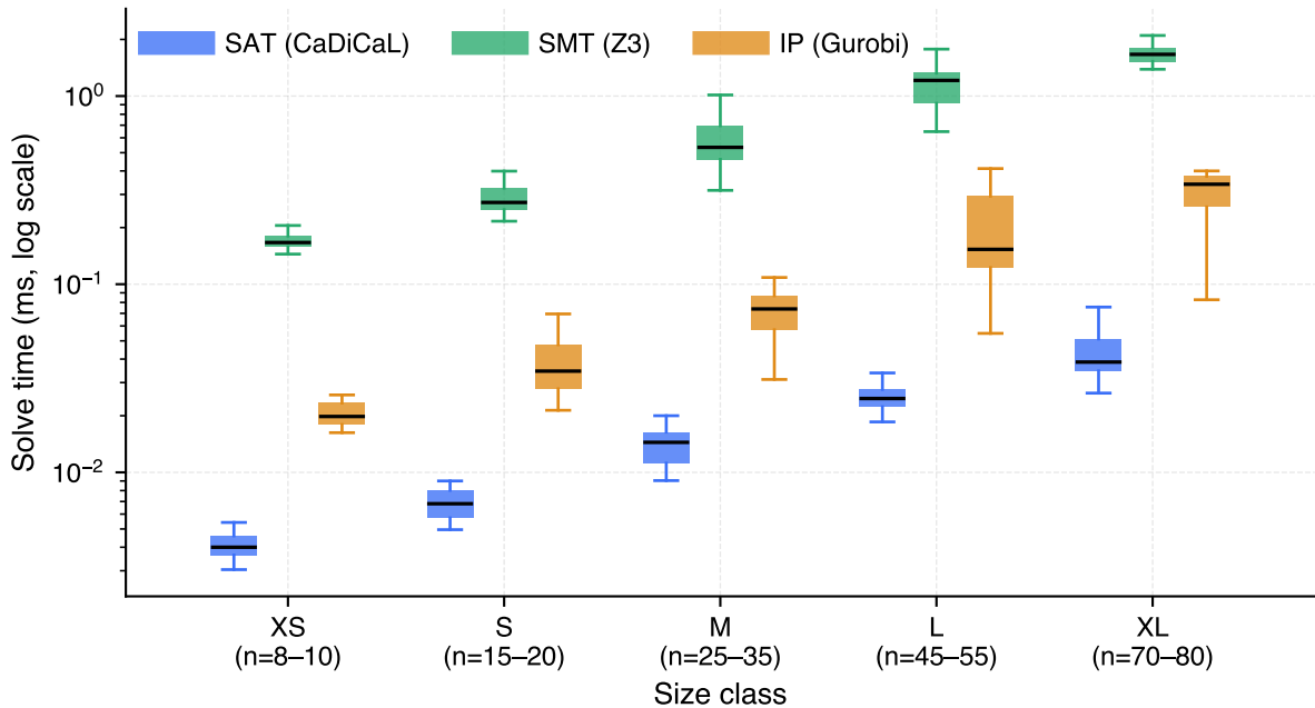
Solve time per encoding across size classes (n=20 each)
