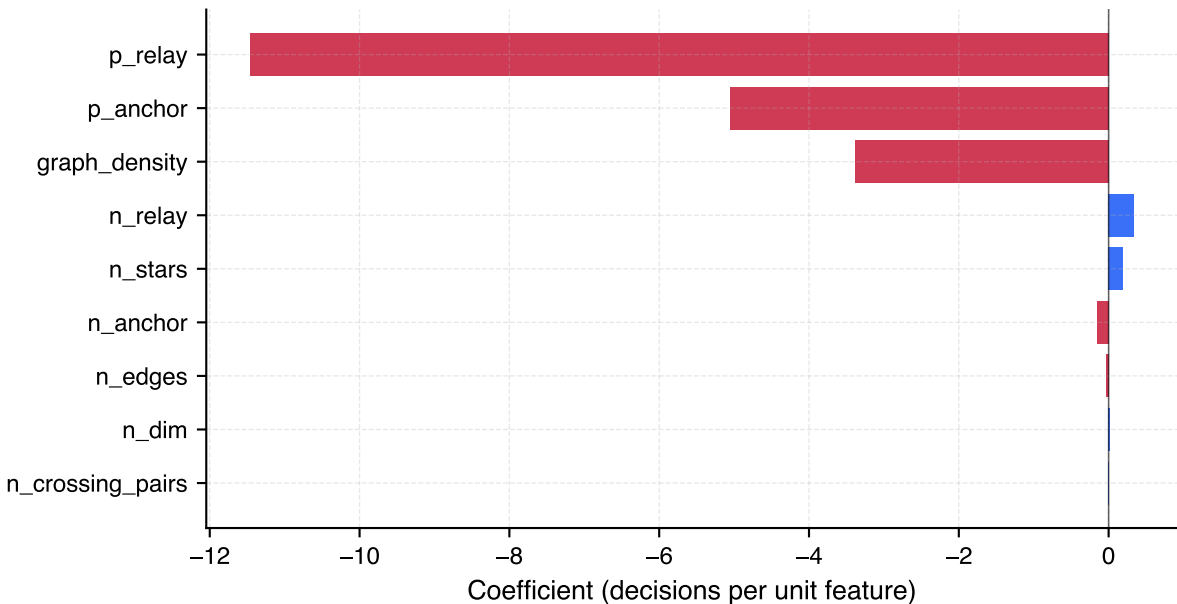
Difficulty regression: features vs solver decisions ( R^2 = 0.156 )
