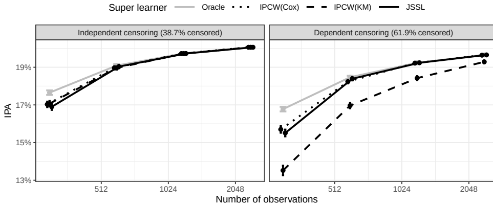
FIGURE 1 For the risk prediction models provided by each of the super learners, the IPA is plotted against sample size (on \log_2 scale). The results are averages across 1000 simulated data sets and the error bars are used to quantify the Monte Carlo uncertainty. JSSL denotes the joint survival super learner.
