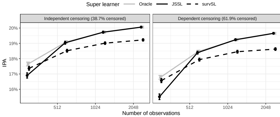
FIGURE 2 For the risk prediction models of the outcome provided by each of the super learners, the IPA at the fixed time horizon is plotted against sample size (on \log_2 scale). The results are averages across 1000 repetitions and the error bars are used to quantify the Monte Carlo uncertainty. JSSL denotes the joint survival super learner.
