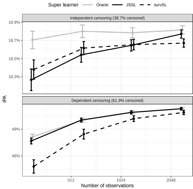
FIGURE 3 For the risk prediction models of the censoring model provided by each of the super learners, the IPA at the fixed time horizon is plotted against sample size (on log 2 scale). The results are averages across 1000 repetitions and the error bars are used to quantify the Monte Carlo uncertainty. JSSL denotes the joint survival super learner.
