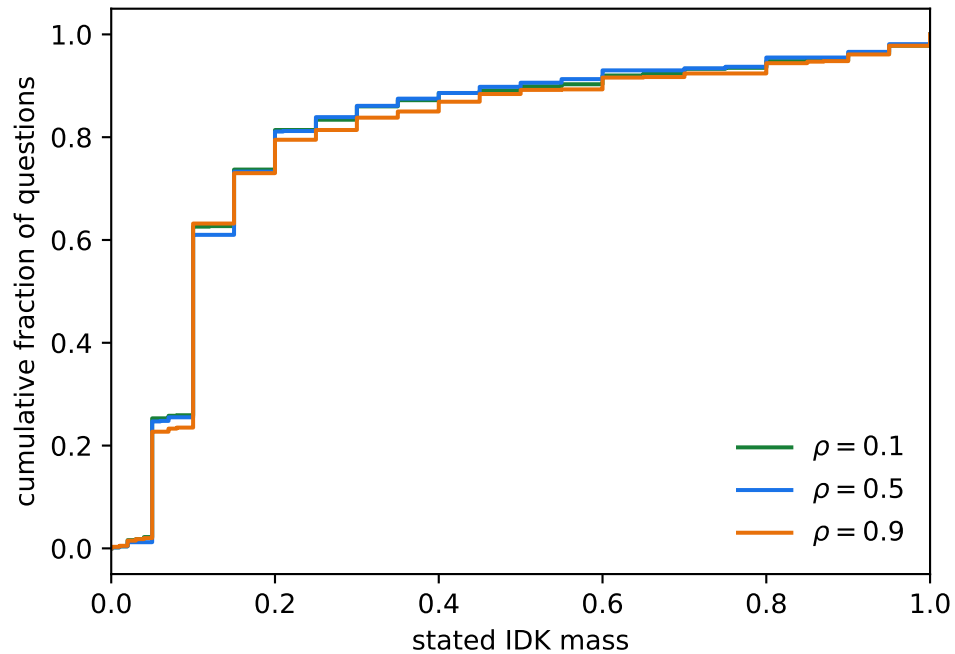
Residual/IDK mass
