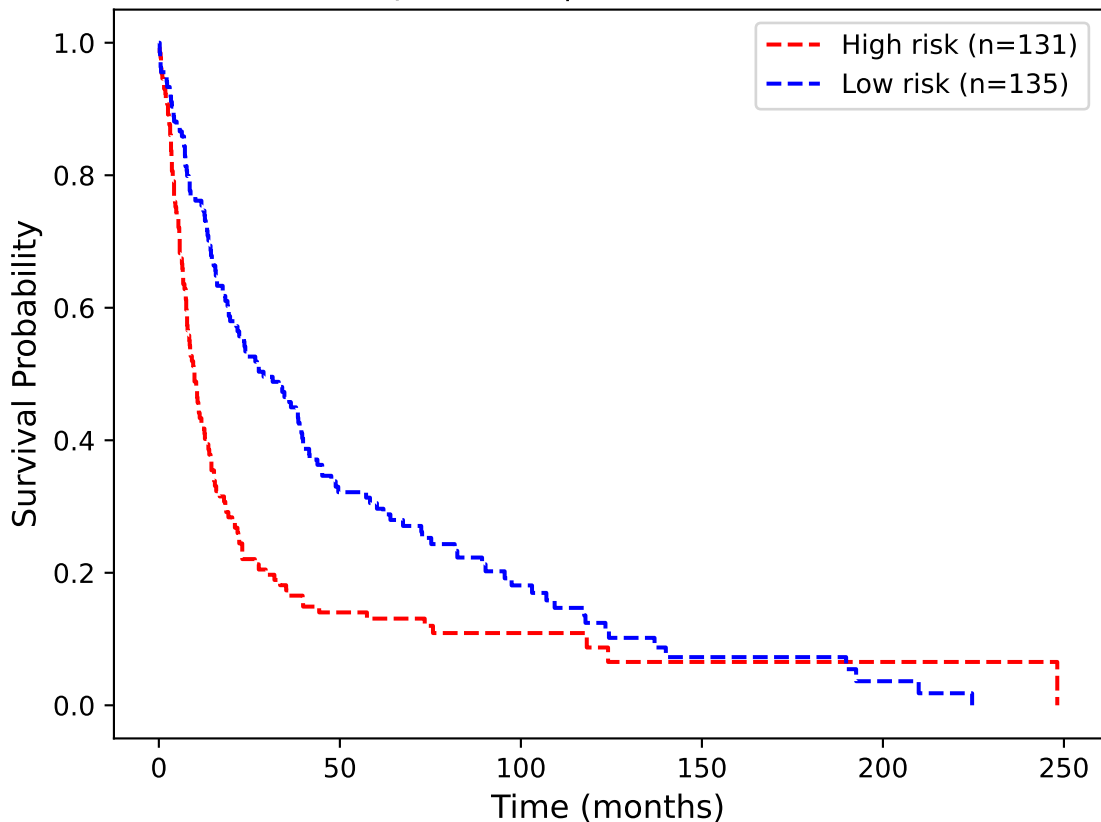
Program Model — Gravendeel p=0.0000 | C-index=0.624
