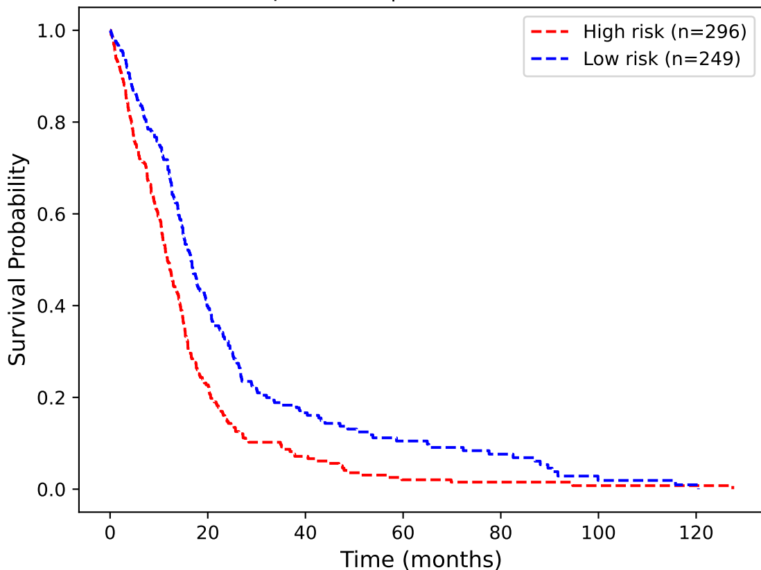
Program Model — TCGA p=0.0000 | C-index=0.610
