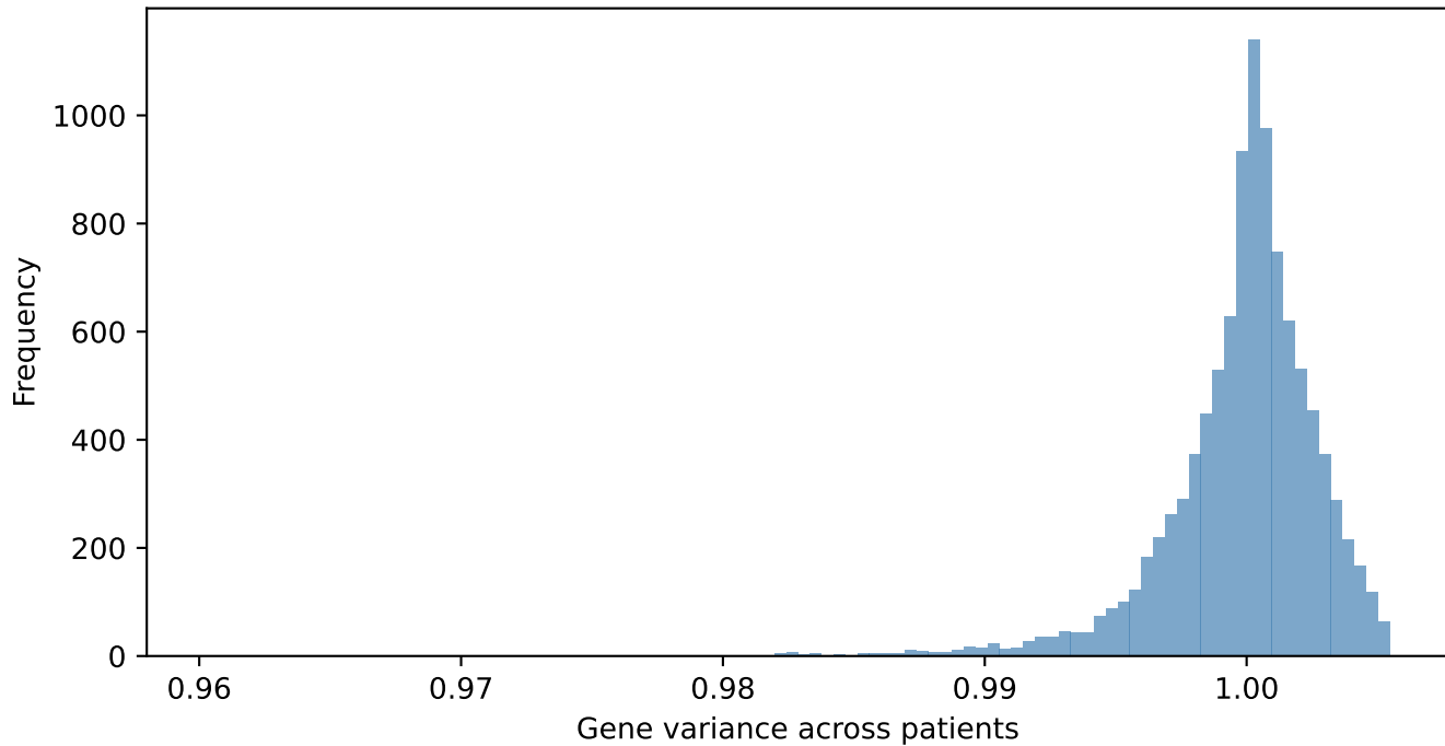
Gene variance distribution
