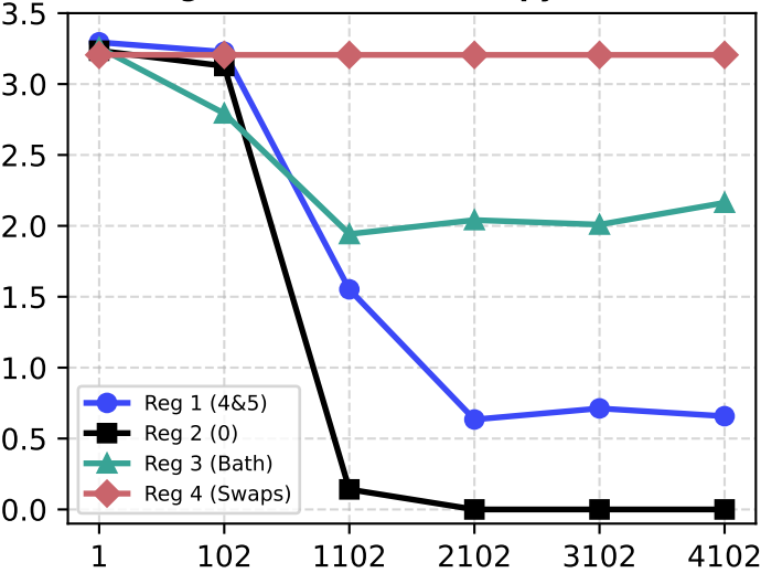
E. Regional Shannon Entropy H(t) (bits)
