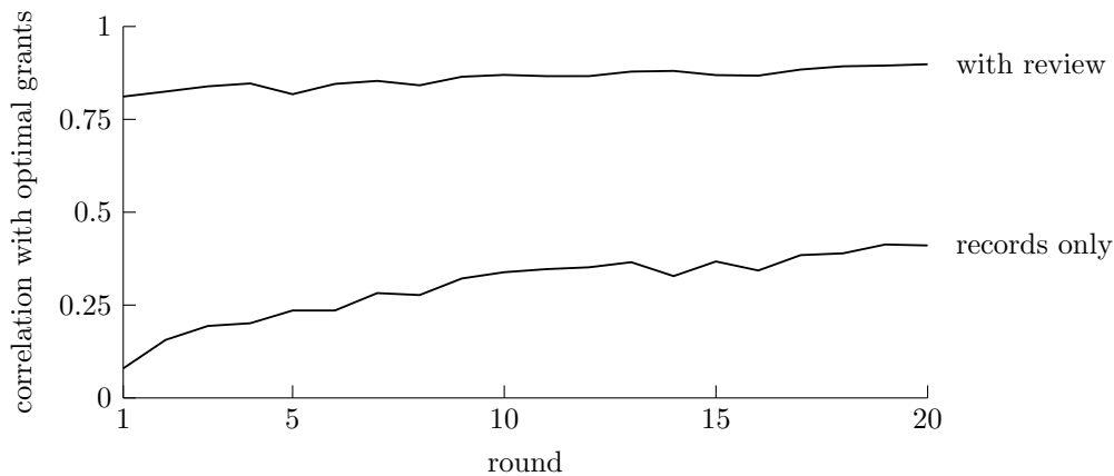
FIGURE 4. Records do not catch up. The correlation of each funder’s grants with the optimal grants, round by round, at the default parameters ( \tau_K = 1 , fifty seeds, twenty rounds). The records-only funder improves slowly, from 0.08 in the first round to 0.41 by round twenty, and remains further from the optimal allocation than the funder with the review signal is in round one (0.81). Under heavy-tailed capability the pattern is the same: 0.07 to 0.43, against 0.92.
