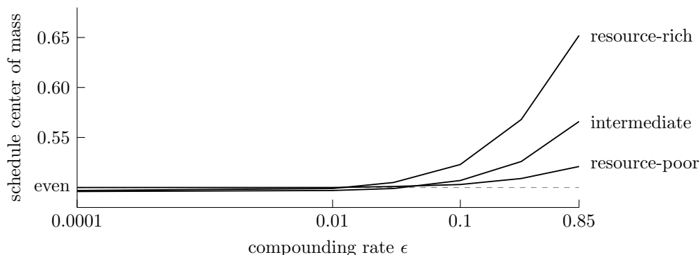
FIGURE 7. Compounding, not poverty, sets the schedule’s tilt. The schedule’s center of mass (0.5 is even; higher is later) as the compounding rate \epsilon increases, for communities of baseline resource scale r_{\min} = 3, 0.3 , and 0.001 . Below \epsilon \approx 0.03 every schedule is within half a percent of even; as compounding increases, every community’s schedule leans later. Resource poverty raises the early share and decreases the intensity of the effect, but does not reverse it. Two hundred seeds per cell.
