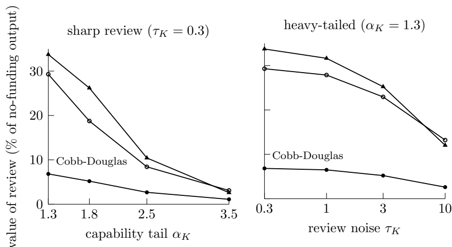
FIGURE 13. The structure of review’s value survives the production technology. The value of the review signal as a percent of no-funding output, across the CES family: at every technology tested, the value increases as capability grows more heavy-tailed (left, decreasing \alpha_K ) and as review grows more informative (right, decreasing \tau_K ), and its scale increases with complementarity. Filled circles: Cobb-Douglas; open circles: \gamma = -3 ; triangles: Leontief. Two rounds; one hundred seeds per point (fifty for Leontief).
