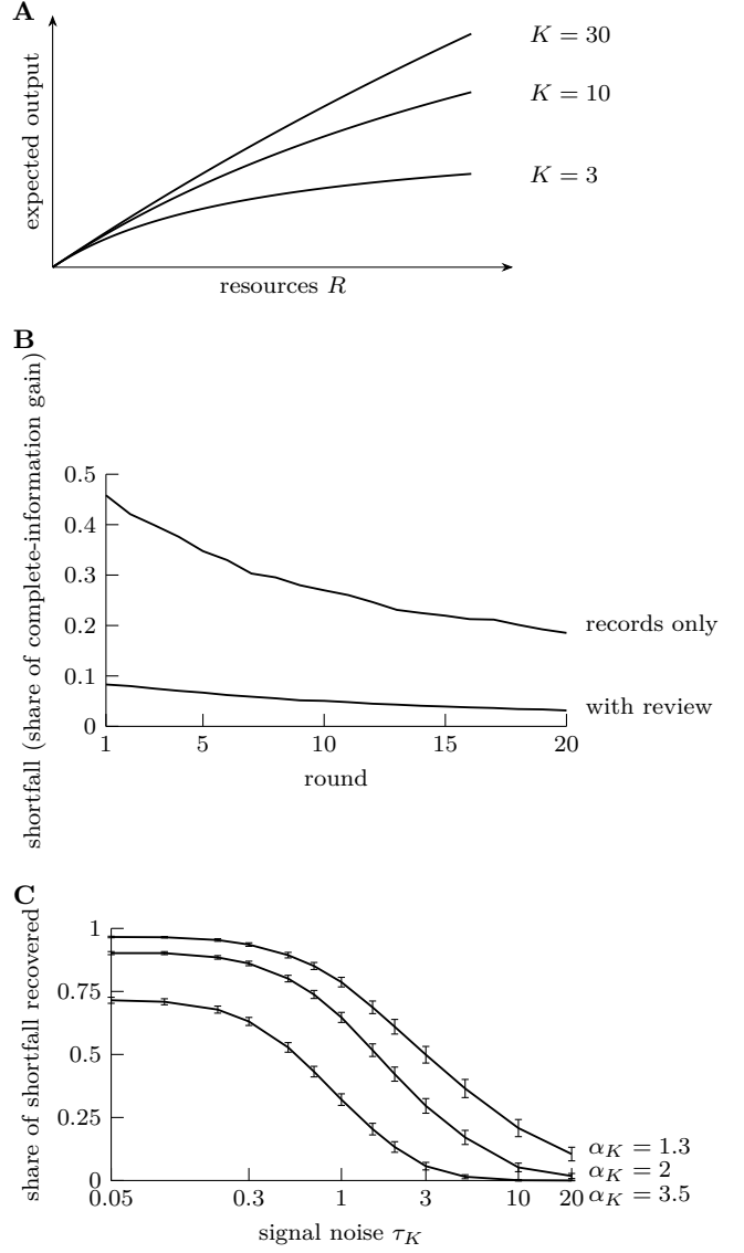
Fig. 2. What the funder can learn. (A) On small grants, research output carries little information about capability: expected output against resources for researchers of capability K = 3, 10 , and 30 ; the curves coincide where resources are small relative to capability. (B) Records do not catch up: the shortfall of each funder's expected output below the complete-information optimum, as a share of what complete-information funding adds, round by round in the default field; the records-only funder's shortfall falls from 46% in round one to 19% by round twenty, while the funder with a single review score observed at the start is at 8% in round one and 3% by round twenty. (C) Review is worth most where capability is heavy-tailed: the share of the records-only shortfall that the review signal recovers, as review noise \tau_K increases, for three capability distributions with the same mean capability (tail parameters \alpha_K = 1.3, 2 , and 3.5 ; mean 2 in each); bars are one standard error over 100 simulated populations. Settings: SI Materials and Methods.
