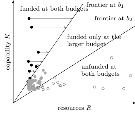
Fig. 1. The gap rule in one population at two budgets. Each point is a researcher, placed by resources and capability. The two lines are the funding frontiers R = cK at a smaller budget b_1 and a larger budget b_2 ; a larger budget raises c and flattens the frontier. Researchers to the left of a frontier are funded at that budget: black points at both budgets, gray points only at the larger budget, open points at neither. Each arrow is a grant at the smaller budget, which moves its researcher exactly to that budget’s frontier; at the larger budget every black and gray researcher receives a grant that moves it to the outer frontier (arrows not drawn).
