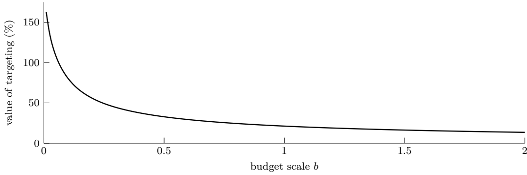
Fig. S2. The value of targeting decreases in the budget. The additional expected output of the optimal allocation over uniform funding, as a fraction of uniform funding's gain over no funding, against the budget scale b , for one population drawn from the default distributions. Corollary 2 proves that the value vanishes as the budget grows; the decrease throughout is a numerical finding (SI Text 1).
