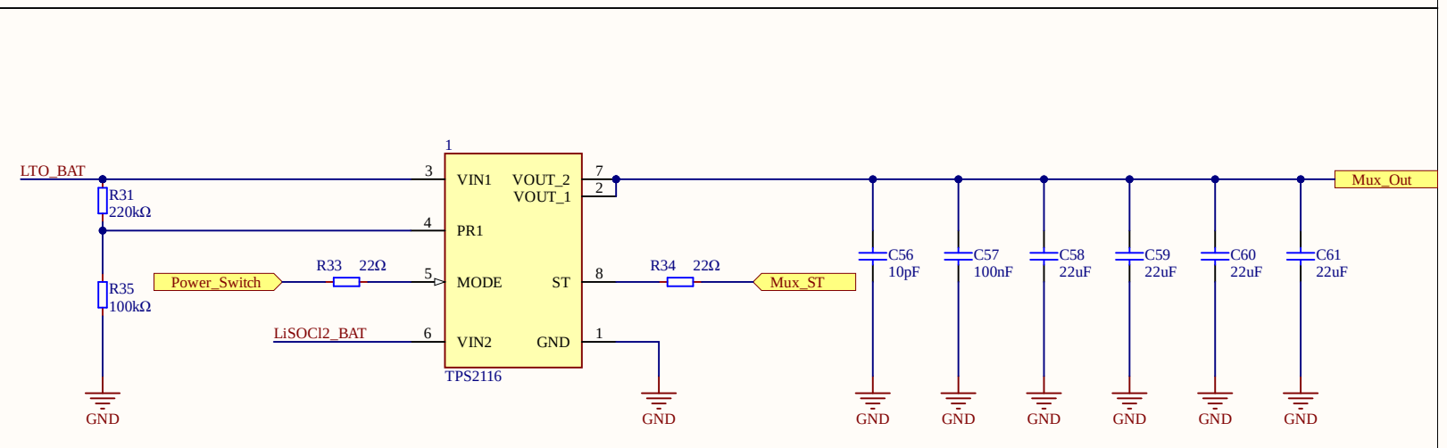
Power Mux w/ Manual mode
