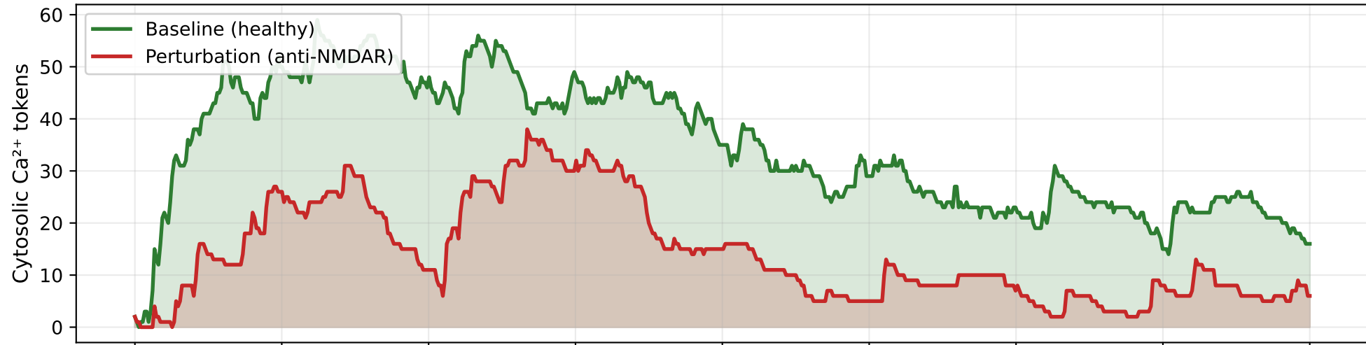
Instantaneous cytosolic Ca 2+ around the NMDAR
