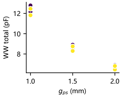
a Cross-winding capacitance
