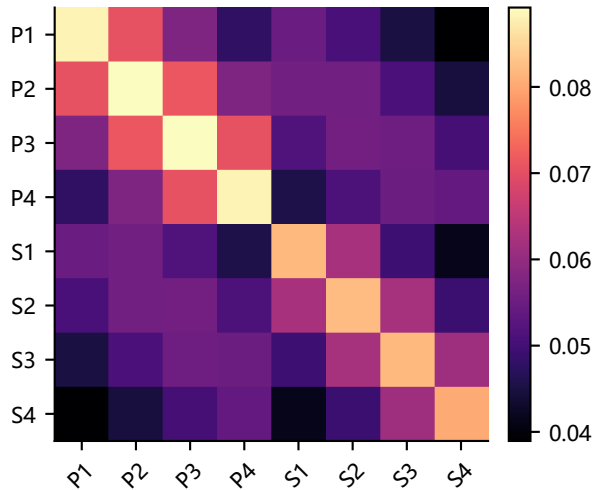
L/M matrix ( \mu\text{H} )
