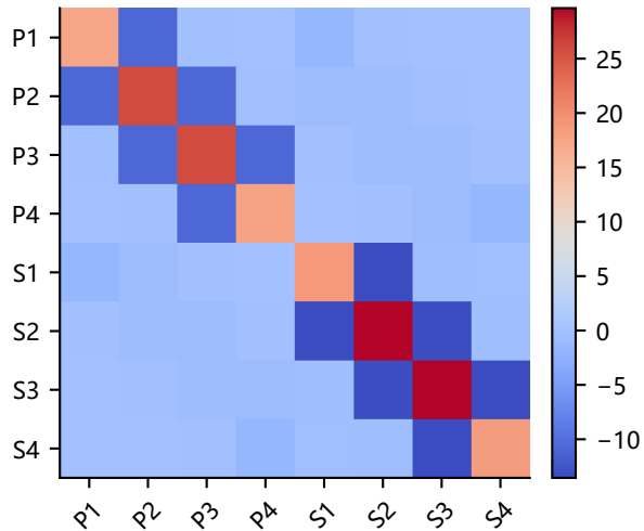
Maxwell C matrix (pF)
