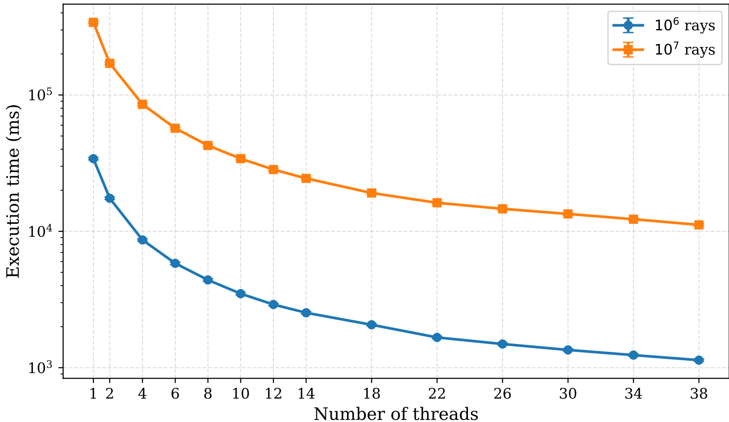
Execution time versus number of threads
