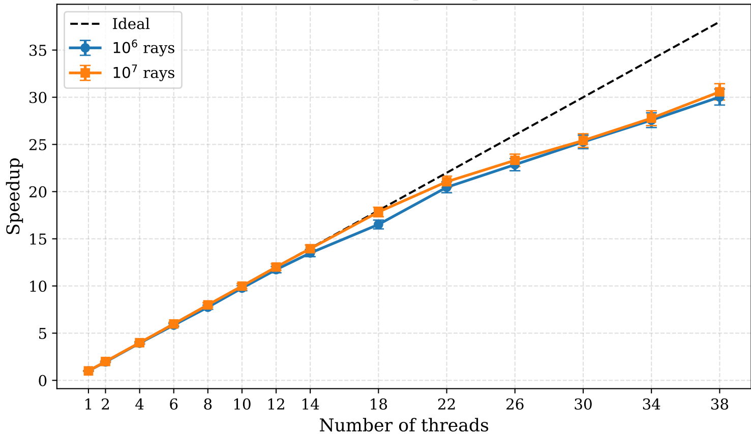
Parallel speedup
