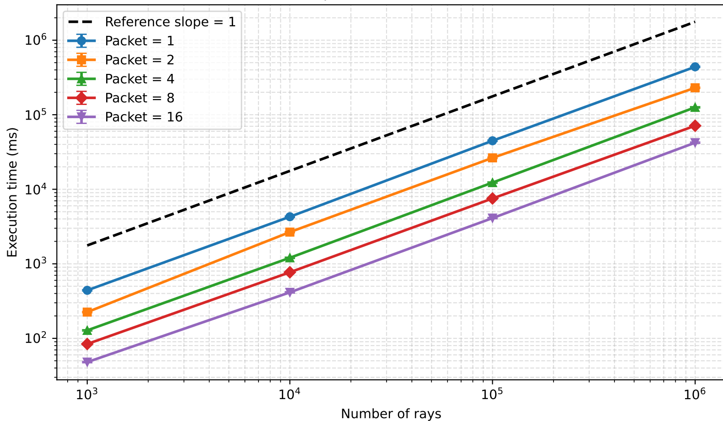
Influence of packet size on execution time
