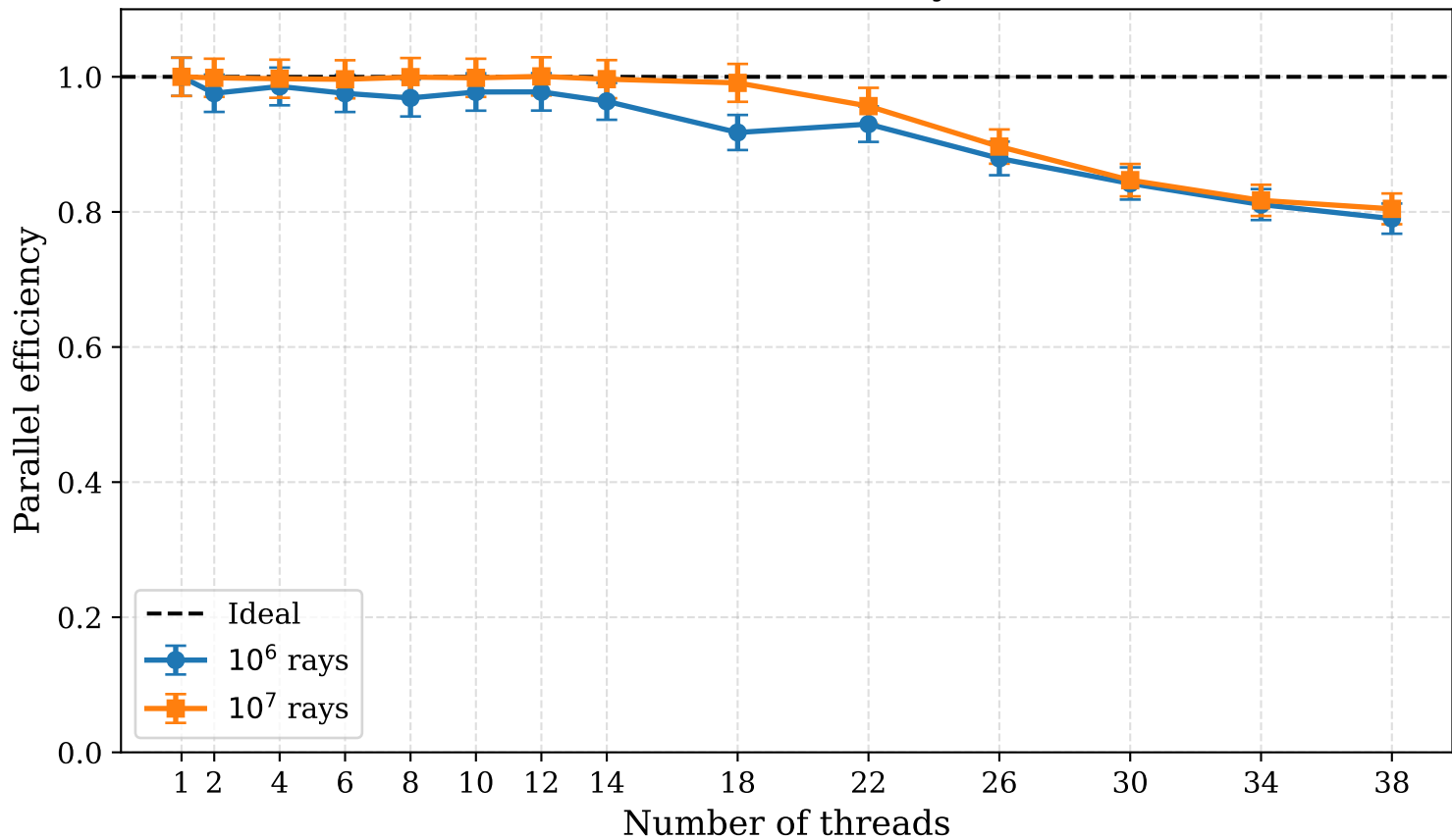
Parallel efficiency
