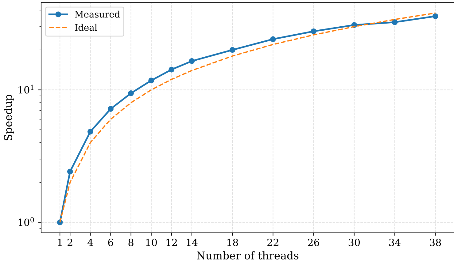
Parallel speedup
