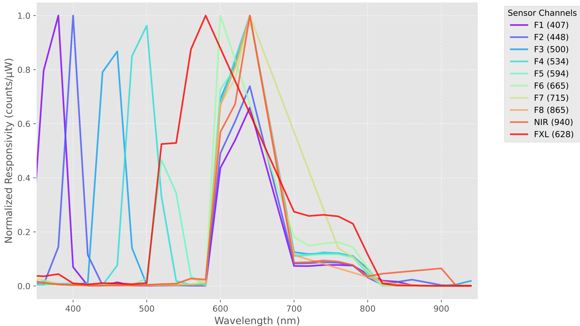
Empirical Spectral Sensitivity Curves (TCS3448 Calibration)
