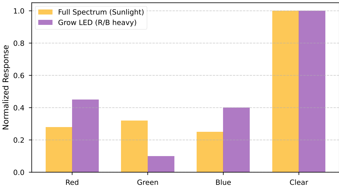
Spectral Signatures: Sunlight vs. Growth LED
