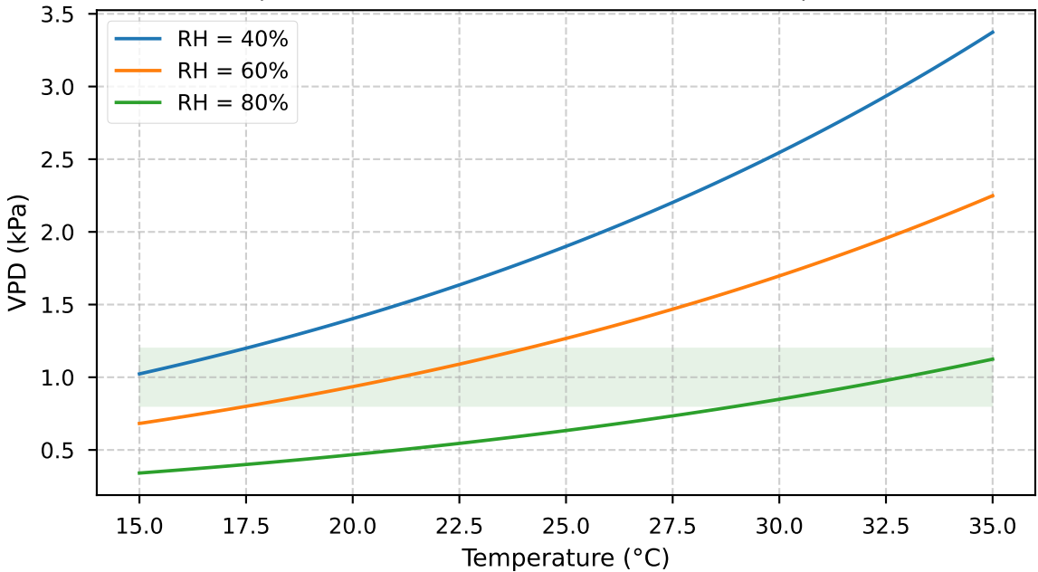
Vapor Pressure Deficit (VPD) as a function of Temperature
