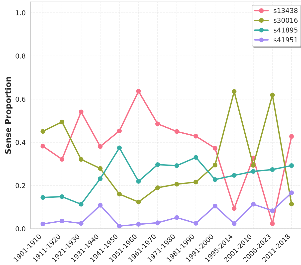
Sense Dominance Over Time: kurs
