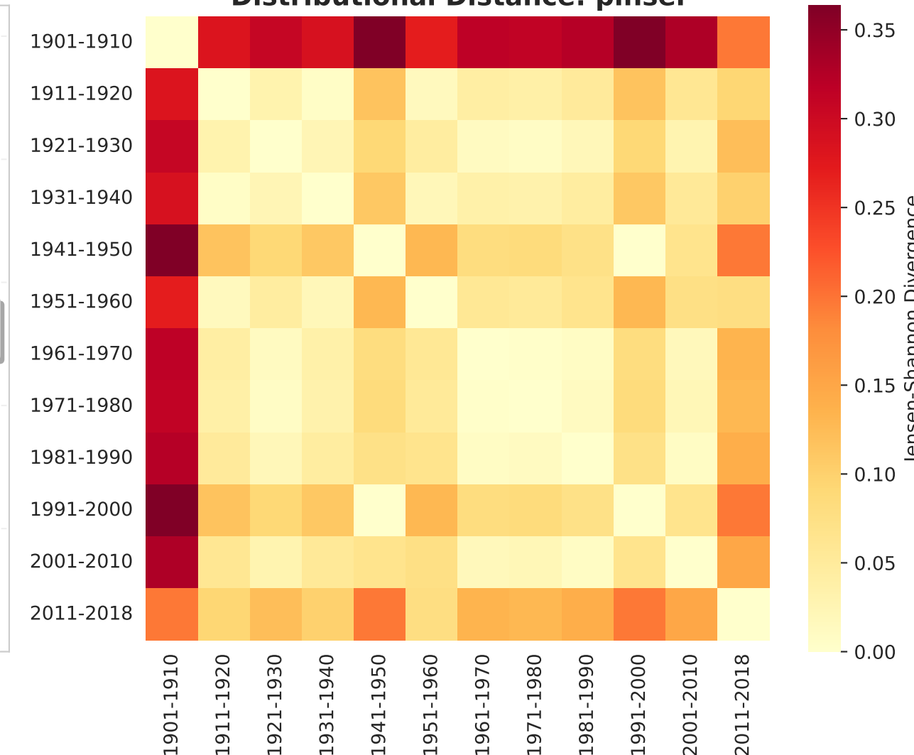
Distributional Distance: pinsel
