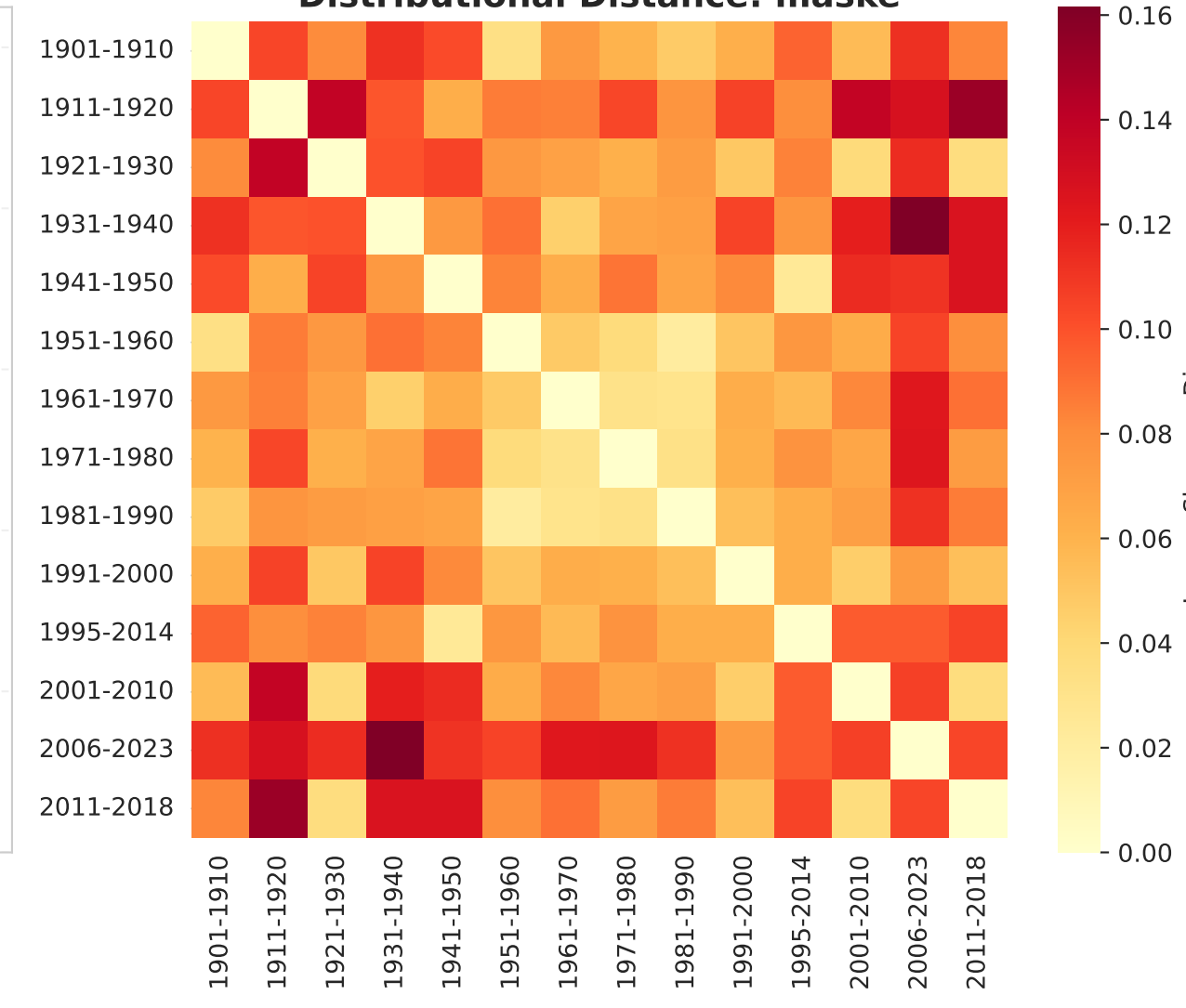
Distributional Distance: maske
