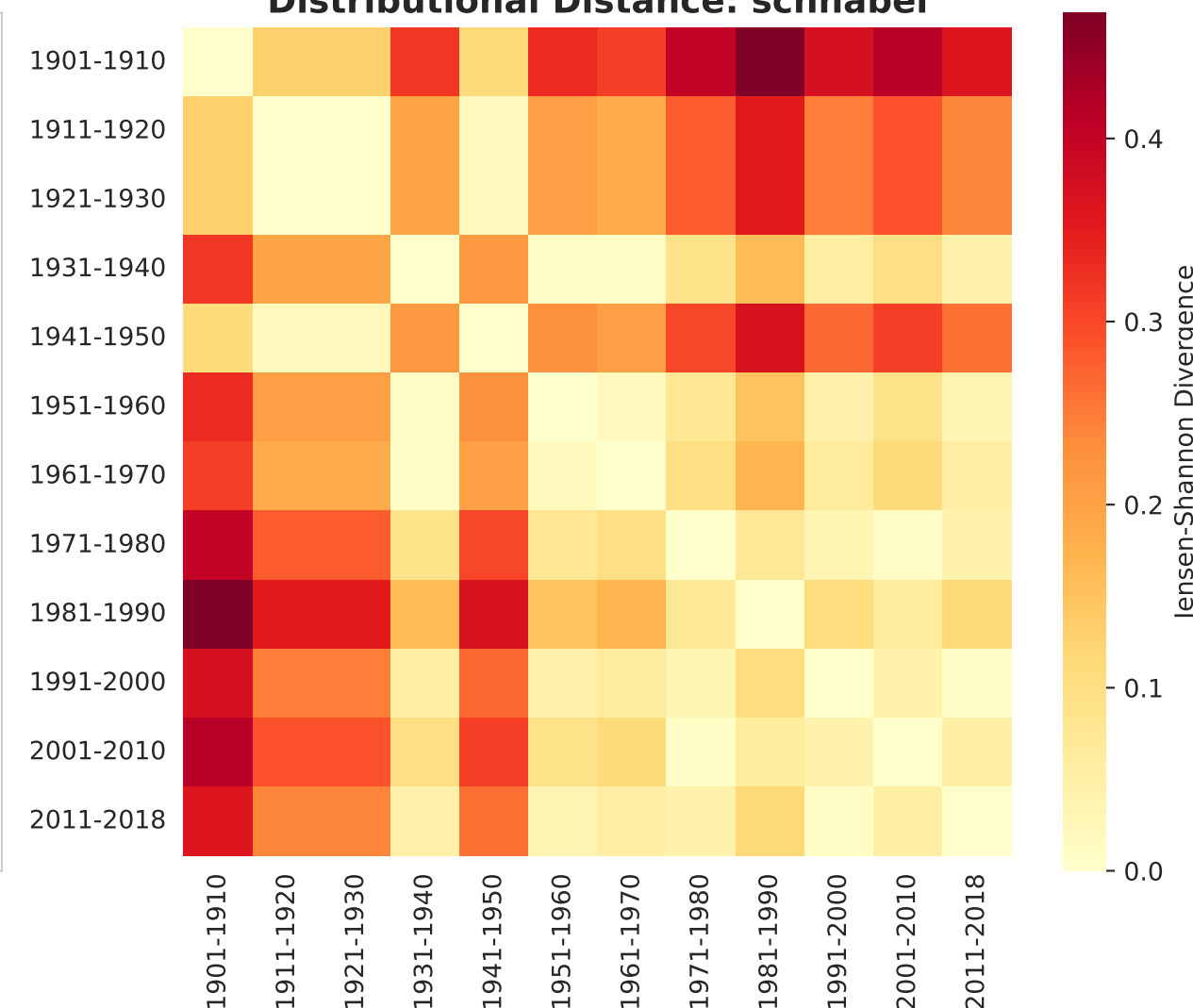
Distributional Distance: schnabel
