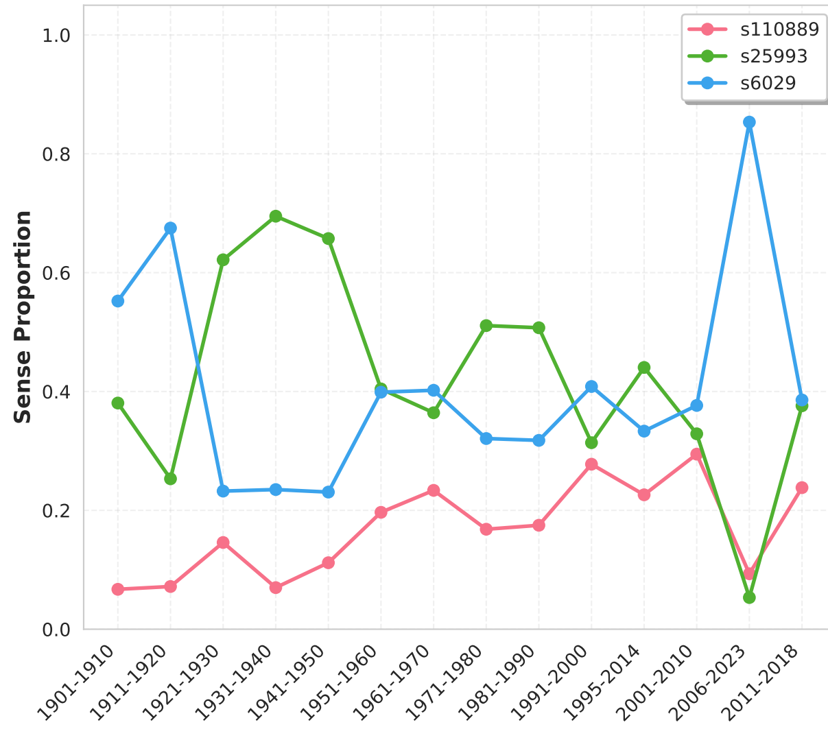
Sense Dominance Over Time: klappe
