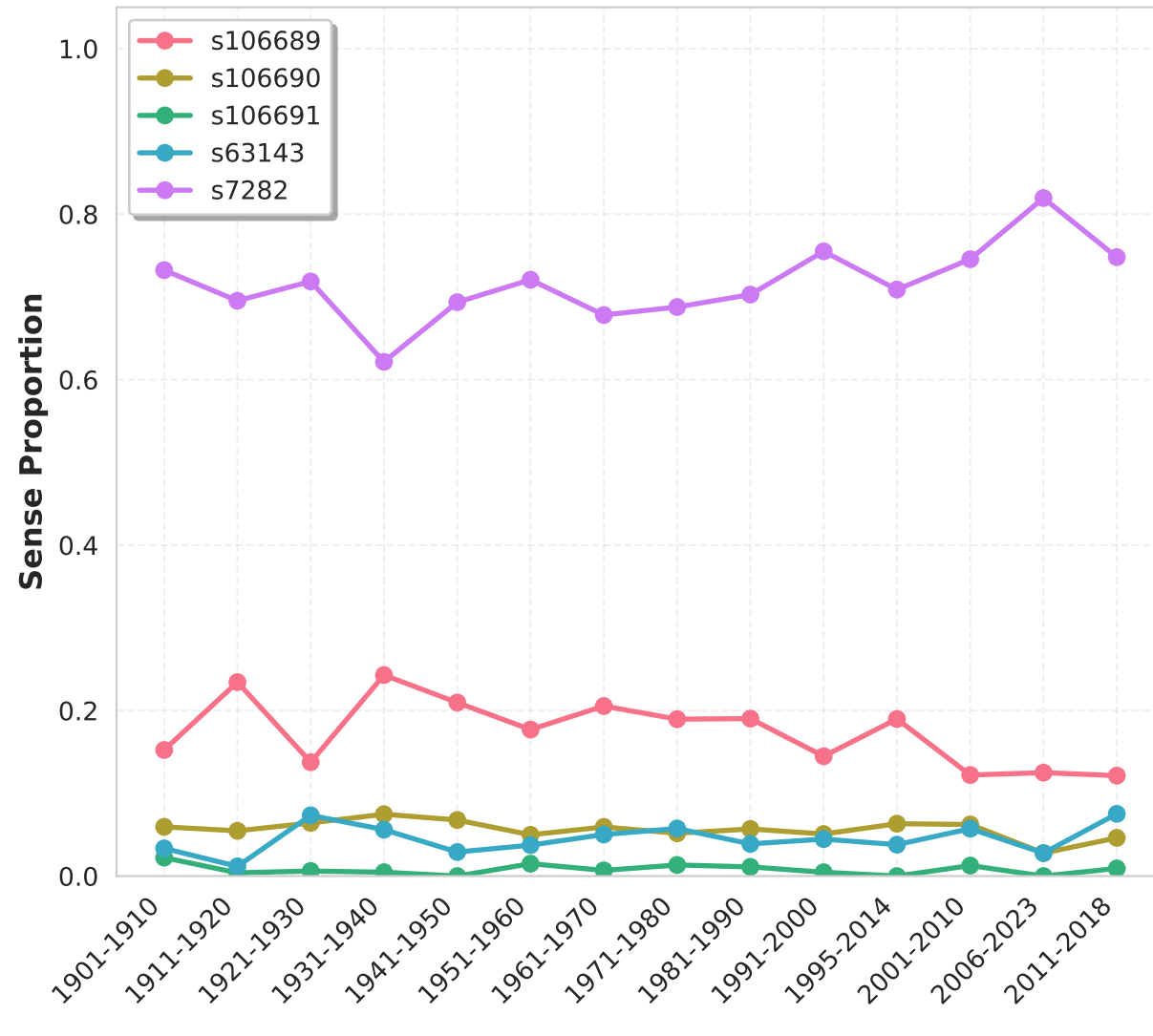
Sense Dominance Over Time: maske
