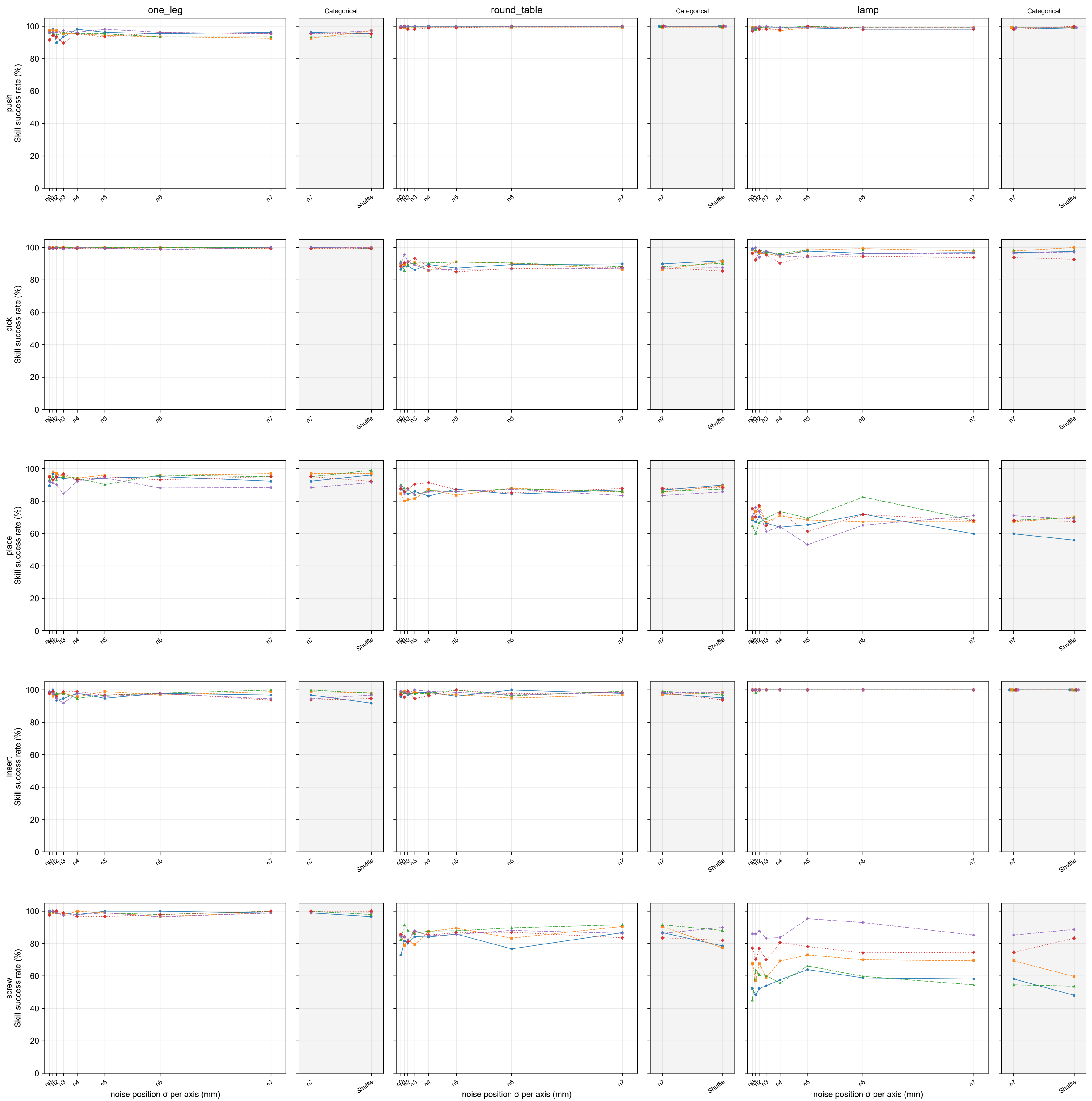
Skill-level skill success rate (%); n0–n7 actual noise scale
