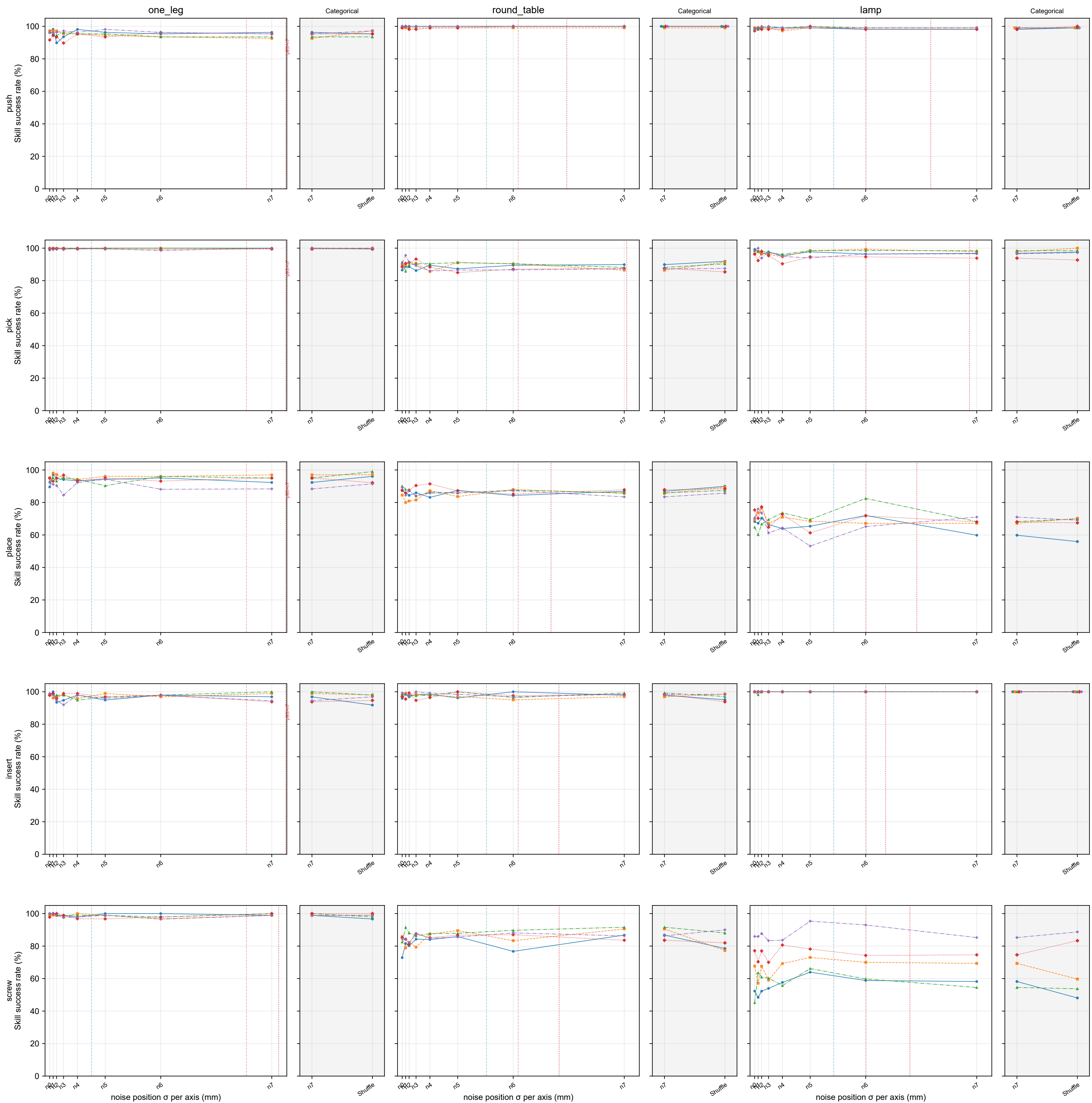
Skill-level success rate; n0–n7 actual noise scale with VLM references
