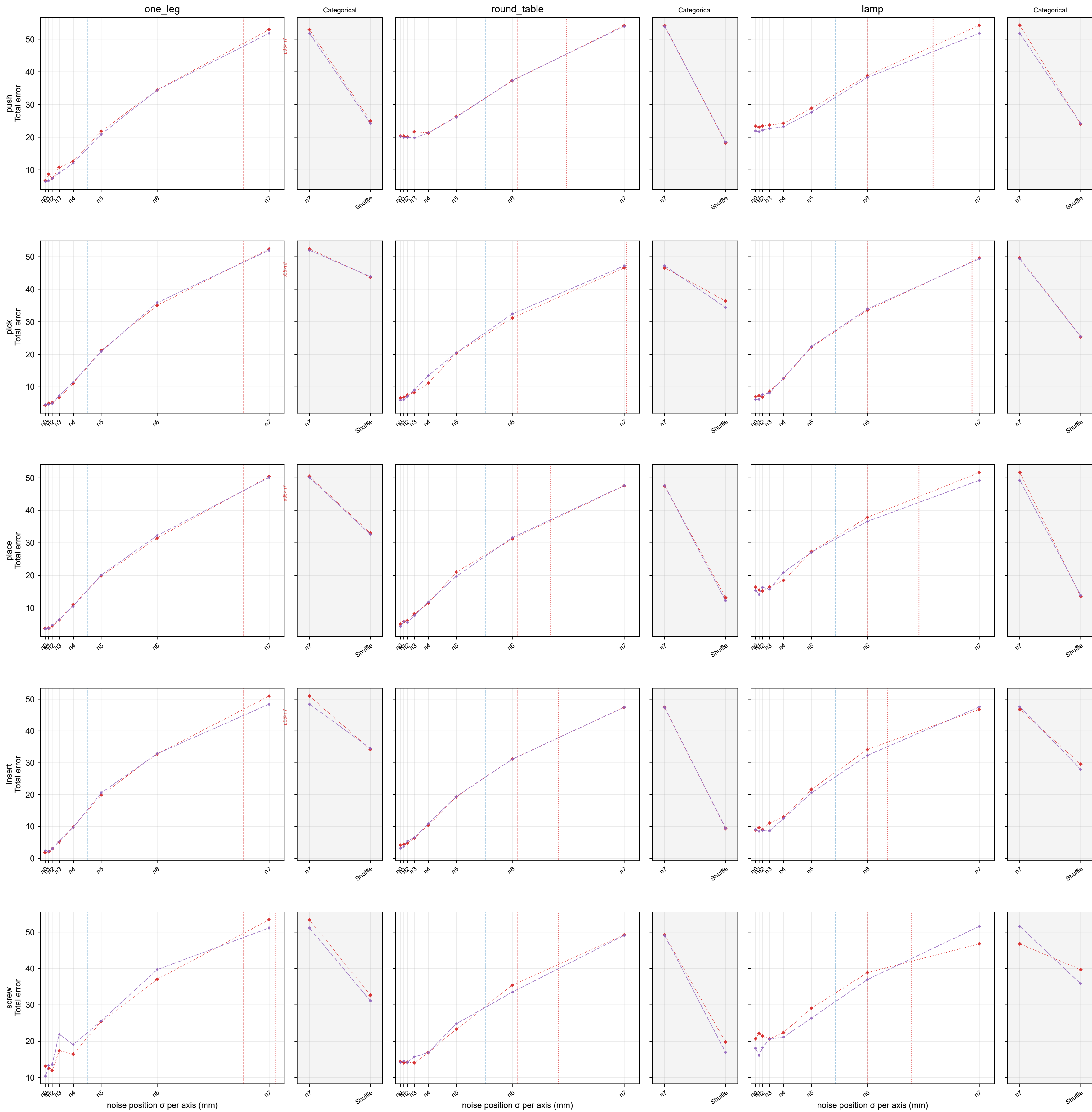
Skill-level total error; n0–n7 actual noise scale with VLM references
