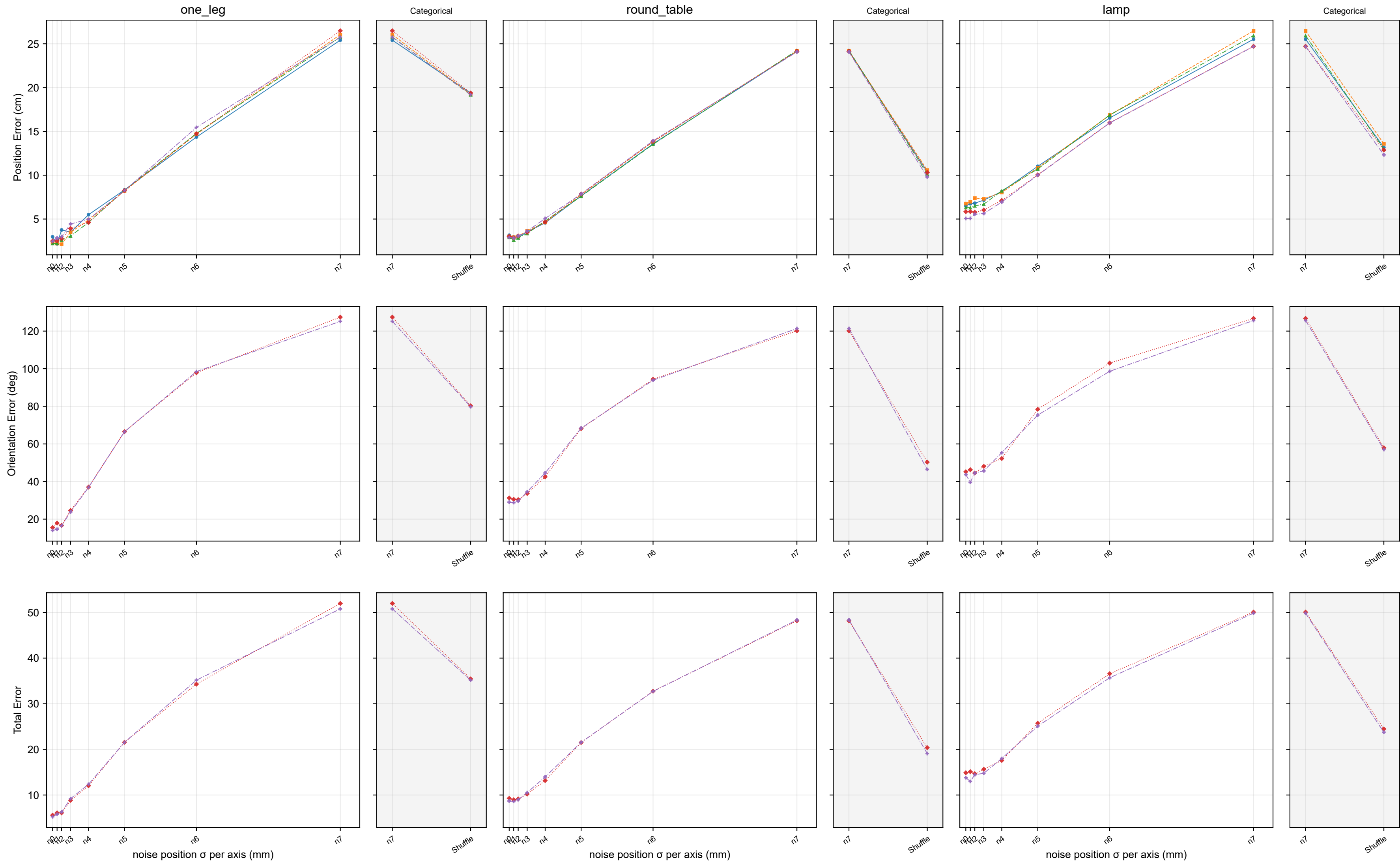
Pooled tracking error curves; position / orientation / total
