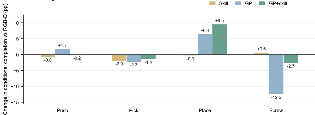
Skill-level changes relative to RGB-D
