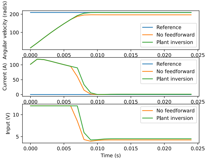
Figure 7.11: Second-order CIM motor response with plant inversion
