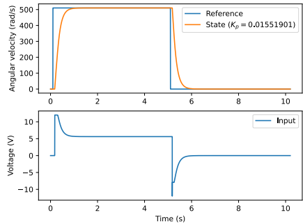
Figure B.6: Flywheel response at 1 ms sample period with 80 ms of output lag (latency-compensated)
