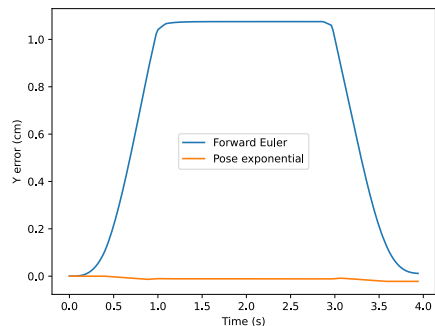
Figure 10.3: Pose estimation comparison (y error vs time)
