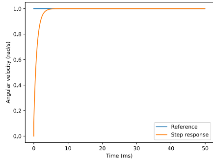
Figure E.6: First-order CIM motor model step response ( L = 0 \mu\text{H} )
