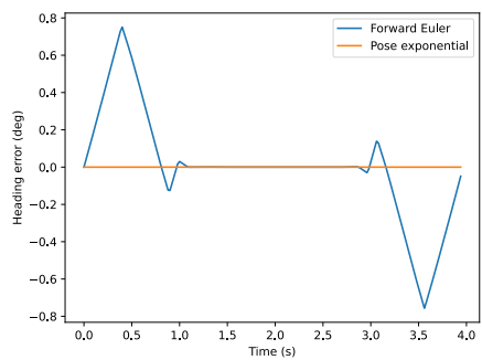
Figure 10.4: Pose estimation comparison (heading error vs time)
