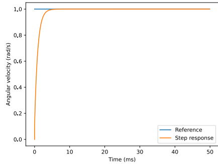
Figure 6.6: Second-order CIM motor model step response ( L = 230 \mu\text{H} ) Figure 6.7: First-order CIM motor model step response ( L = 0 \mu\text{H} )
