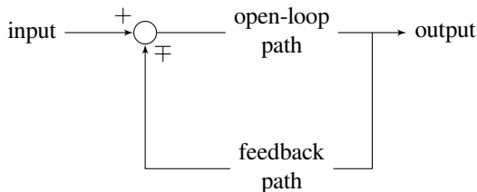
Figure 1.2: Block diagram with nomenclature
