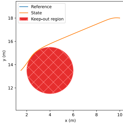
Figure 17.5: Differential drive MPC x-y plot
