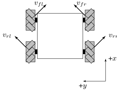
Figure 11.3: Mecanum drive free body diagram
