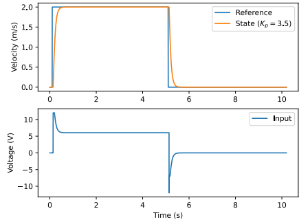
Figure B.4: Drivetrain velocity response at 1 ms sample period with 40 ms of output lag (latency-compensated)
