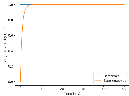
Figure E.16: First-order CIM motor model step response ( L = 0 \mu\text{H} )
