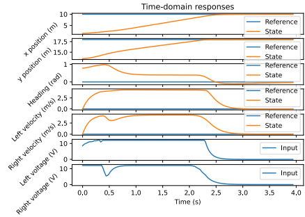
Figure 17.6: Differential drive MPC response
