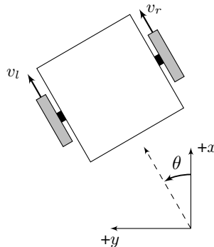
Figure 12.7: Differential drive system diagram
