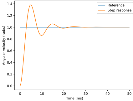
Figure E.15: Second-order CIM motor model step response ( L = 230 \mu\text{H} )
