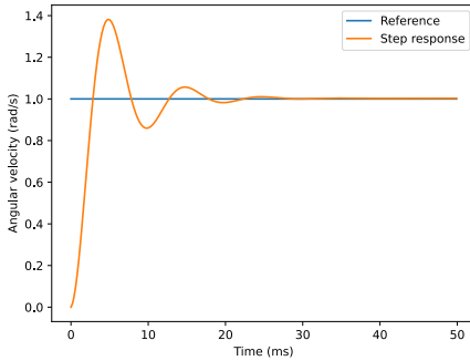
Figure E.5: Second-order CIM motor model step response ( L = 230 \mu\text{H} )
