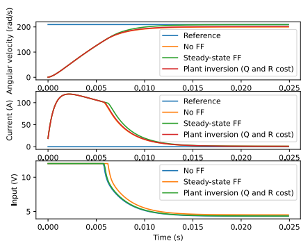
Figure C.2: Second-order CIM motor response with various feedforwards
