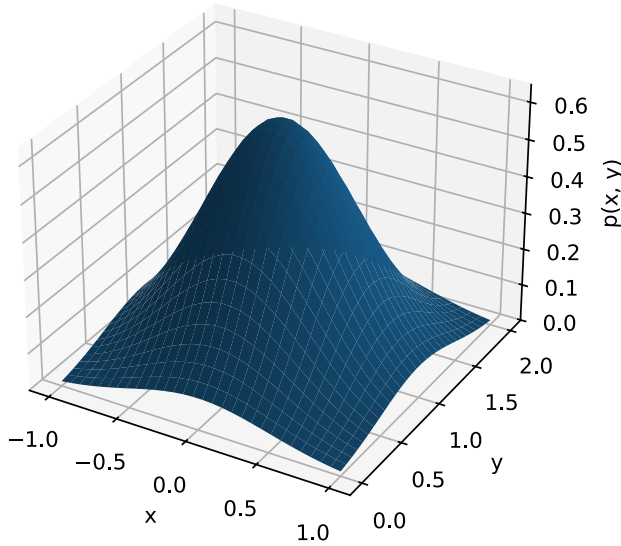
Figure 9.2: Joint probability density function
