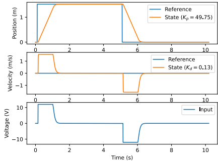
Figure B.2: Elevator response at 5 ms sample period with 50 ms of output lag (latency-compensated)
