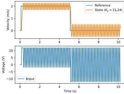
Figure B.3: Drivetrain velocity response at 1 ms sample period with 40 ms of output lag
