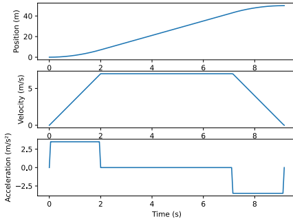
Figure 15.1: Trapezoid profile
