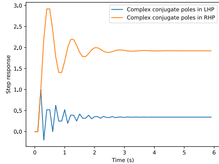
Figure E.20: Complex conjugate poles in various locations in z-plane
