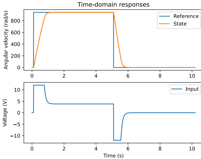
Figure 17.4: Flywheel MPC response
