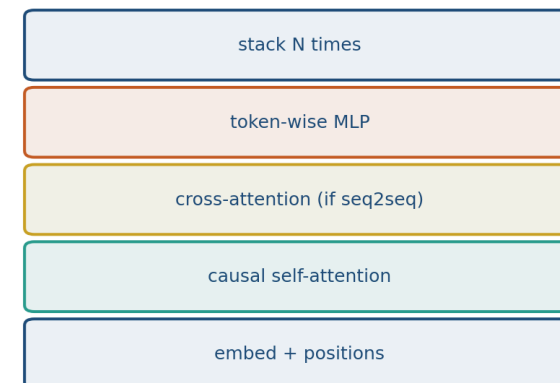
Decoder (GPT drops cross-attention)
