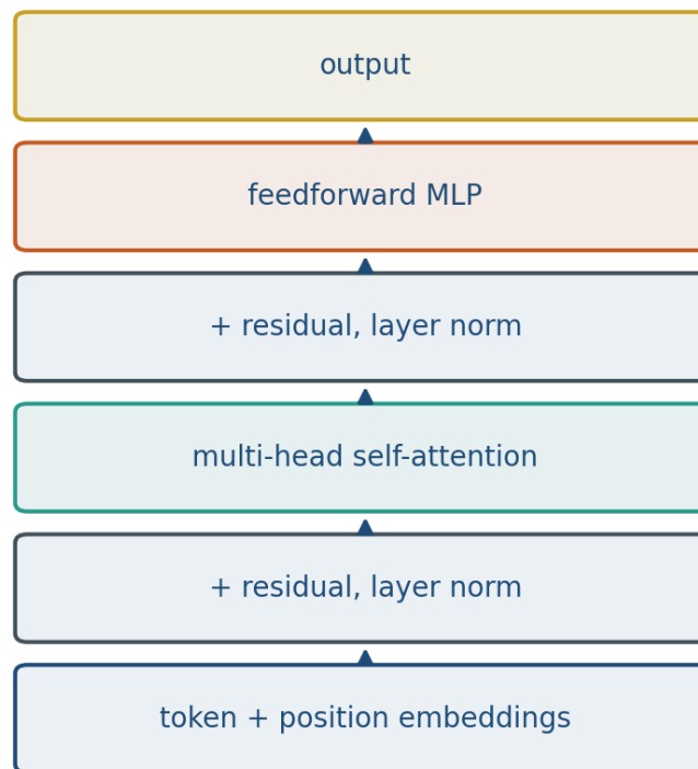
One transformer block
