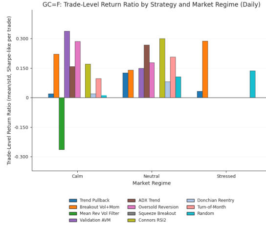
Grouped bars compare trade-level return ratio (mean return / return std. Sharpe-like per trade, not annualized Sharpe) across calm, neutral, and stressed regimes. Light gray bars denote regime cells suppressed for low sample size (fewer than 5 trades). Suppressed cells in this figure: 11.
