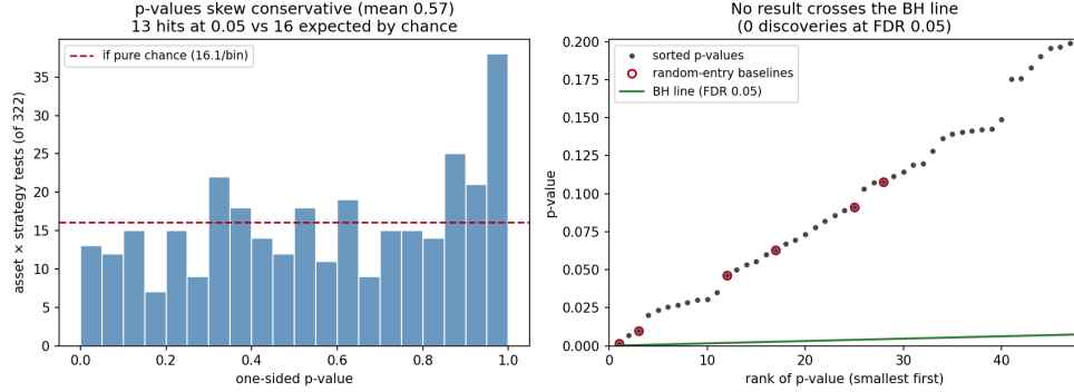
Figure 7: Cross-asset panel of 322 structure-preserving tests across 47 instruments. Left: the p -value histogram skews conservative, with 13 nominal rejections versus 16.1 expected by chance. Right: the Benjamini–Hochberg plot—no ordered p -value crosses the FDR line, so there are zero discoveries; circled points are random-entry baselines, which sit among the smallest p -values.
