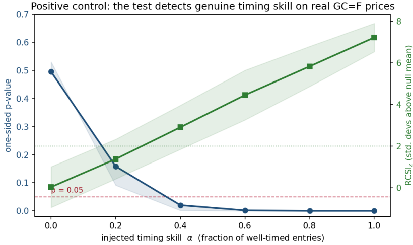
Figure 3: Positive control on real GC=F prices. As injected timing skill \alpha increases, the mean one-sided p -value (blue, left axis) collapses below 0.05 and the mean \text{RCSI}_z (green, right axis) rises well past 2. Bands show the seed dispersion. At \alpha = 0 the test behaves like the null.
