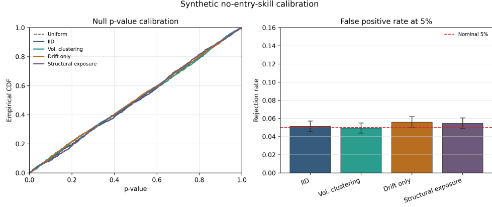
Figure 1: Synthetic p-value calibration under no-entry-skill worlds. The left panel compares empirical p-value CDFs with the uniform benchmark; the right panel reports false positive rates at the 5% level.
