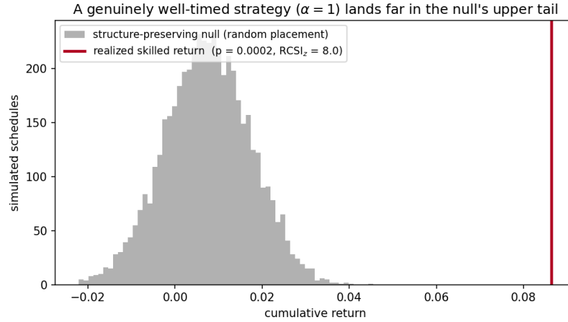
Figure 4: A single genuinely well-timed strategy ( \alpha = 1 ) on the real GC=F path. The realized cumulative return (red) lies far beyond the entire structure-preserving null distribution of the same trades placed at random ( p \approx 0.0002 , RCSI_z \approx 8 ).
