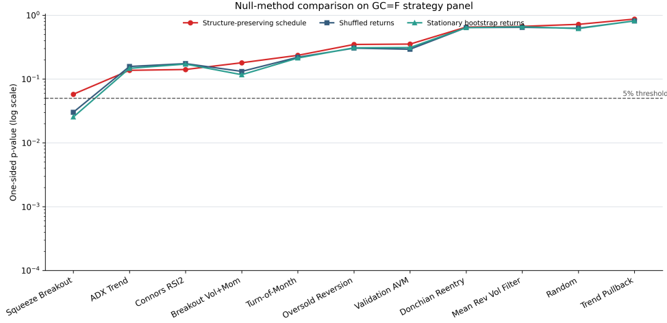
Figure 5: One-sided p-values under structure-preserving schedule randomization, shuffled returns, and stationary-bootstrap returns.
