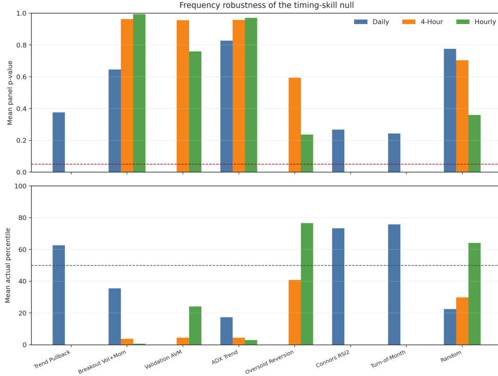
Figure 8: Frequency-robustness check across recent daily, 4-hour, and hourly panels. The top panel reports mean panel p -value by strategy and interval; the bottom panel reports mean actual percentile.
