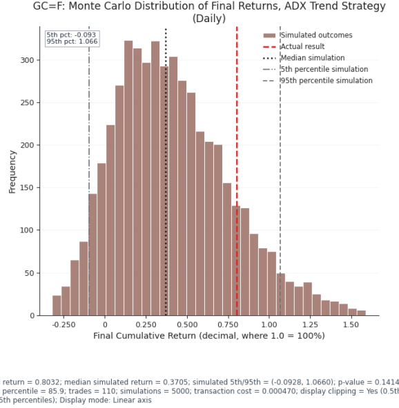
Figure 16: GC=F. Monte Carlo distribution of final returns, ADX Trend (daily). Caption values: actual return = 0.8032; median simulated return = 0.3705; simulated 5th/95th = (-0.0928, 1.0660); p-value = 0.1414; actual percentile = 85.9; trades = 110; simulations = 5,000; transaction cost = 0.000470.
