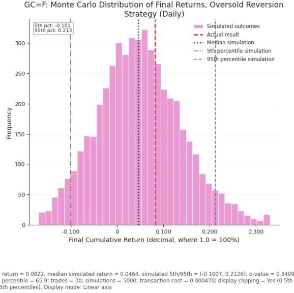
Figure 17: GC=F. Monte Carlo distribution of final returns, Oversold Reversion (daily). Caption values: actual return = 0.0822; median simulated return = 0.0464; simulated 5th/95th = (-0.1007, 0.2126); p-value = 0.3409; actual percentile = 65.9; trades = 30; simulations = 5,000; transaction cost = 0.000470.
