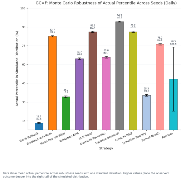
Figure 24: GC=F. Monte Carlo robustness of actual percentile across seeds (daily). Mean \pm SD across outer runs. Examples: Squeeze Breakout 94.3 \pm 0.3 ; ADX Trend 86.2 \pm 0.4 ; Breakout Vol+Mom 82.7 \pm 0.5 ; Random 48.3 \pm 25.6 .
