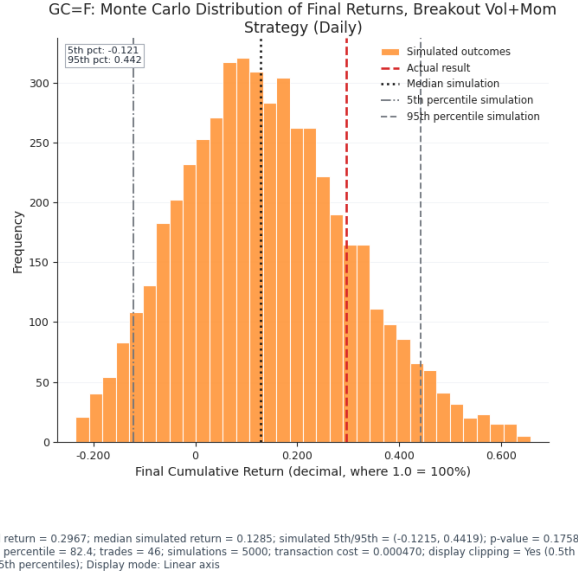
Figure 13: GC=F. Monte Carlo distribution of final returns, Breakout Vol+Mom (daily). Caption values: actual return = 0.2967; median simulated return = 0.1285; simulated 5th/95th = (-0.1215, 0.4419); p-value = 0.1758; actual percentile = 82.4; trades = 46; simulations = 5,000; transaction cost = 0.000470.
