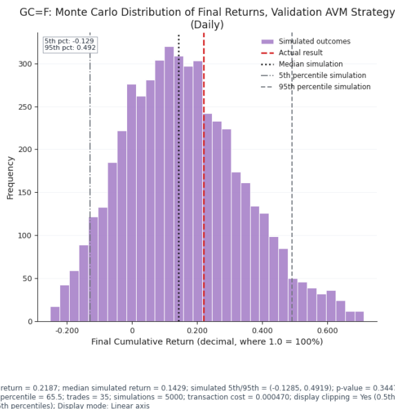
Figure 15: GC=F. Monte Carlo distribution of final returns, Validation AVM (daily). Caption values: actual return = 0.2187; median simulated return = 0.1429; simulated 5th/95th = (-0.1285, 0.4919); p-value = 0.3447; actual percentile = 65.5; trades = 35; simulations = 5,000; transaction cost = 0.000470.
