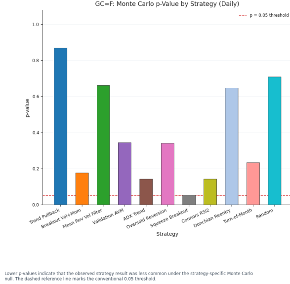
Figure 25: GC=F. Monte Carlo p-value by strategy (daily). The dashed reference line marks the conventional threshold p = 0.05 . None of the plotted p-values crosses this threshold.
