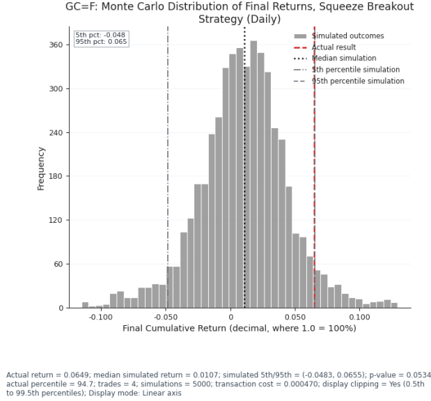
Figure 18: GC=F. Monte Carlo distribution of final returns, Squeeze Breakout (daily). Caption values: actual return = 0.0649; median simulated return = 0.0107; simulated 5th/95th = (-0.0483, 0.0655); p-value = 0.0534; actual percentile = 94.7; trades = 4; simulations = 5,000; transaction cost = 0.000470.
