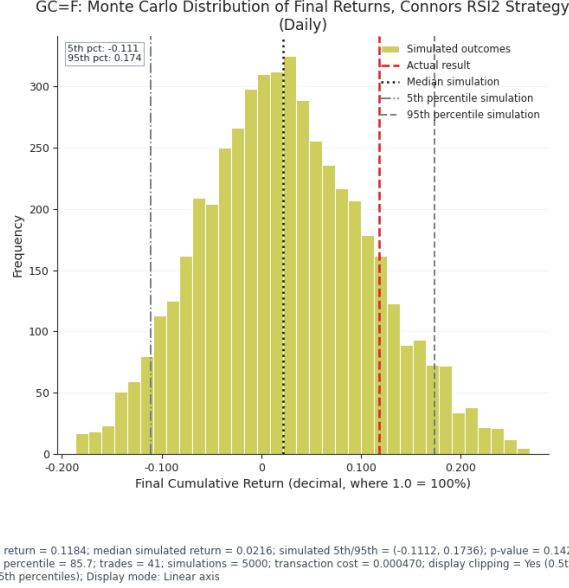
Figure 19: GC=F. Monte Carlo distribution of final returns, Connors RSI2 (daily). Caption values: actual return = 0.1184; median simulated return = 0.0216; simulated 5th/95th = (-0.1112, 0.1736); p-value = 0.1428; actual percentile = 85.7; trades = 41; simulations = 5,000; transaction cost = 0.000470.
