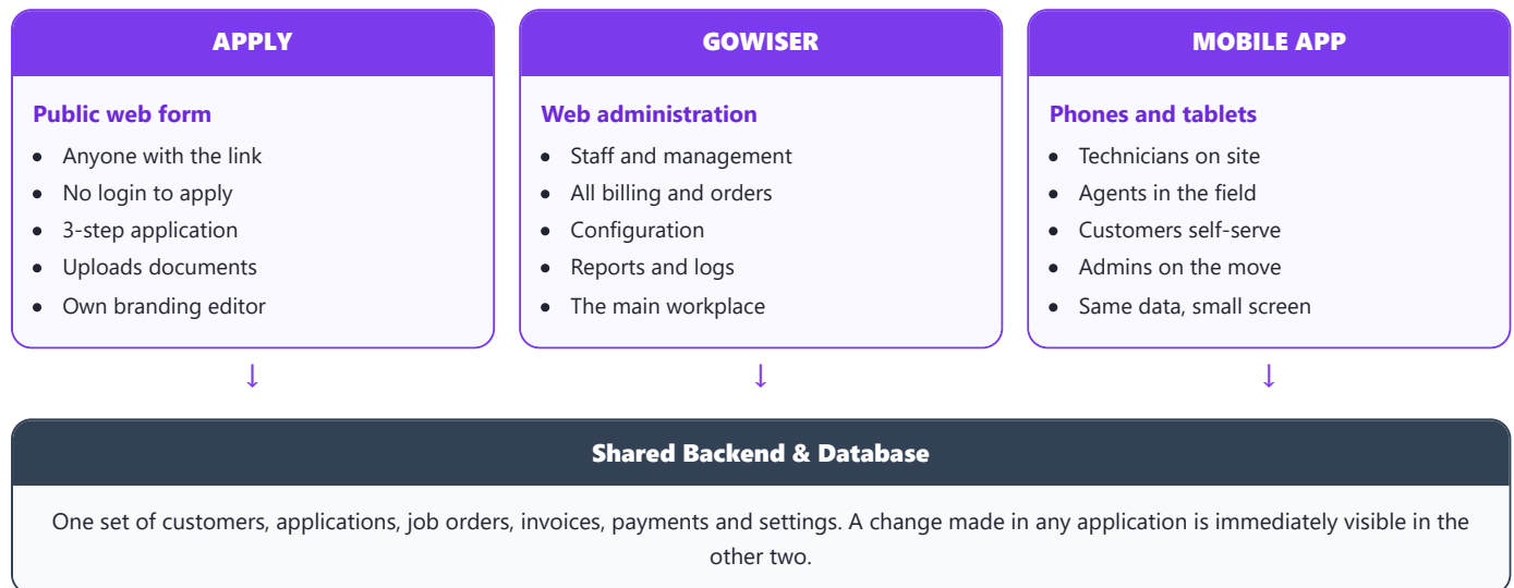
Figure 1. How the three applications fit together.
