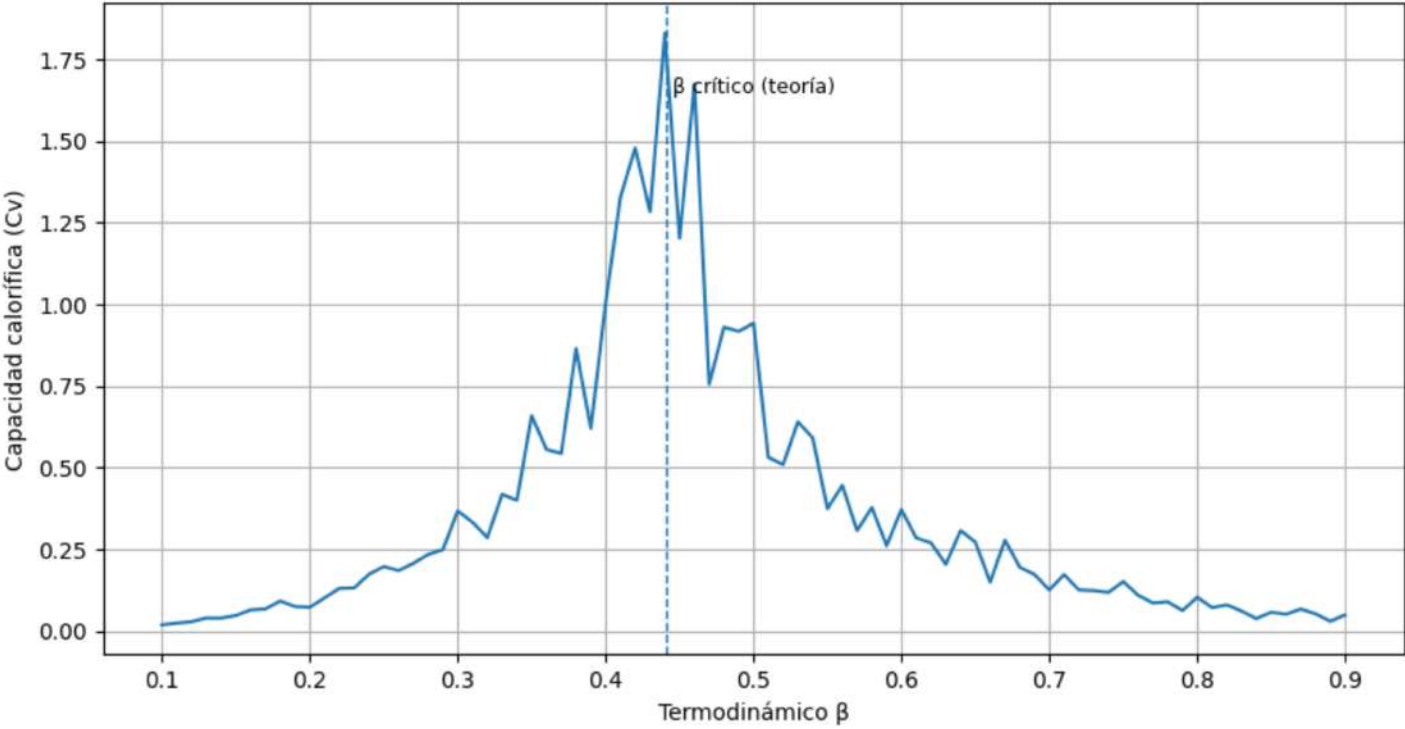
C_v(\beta) - Ising 2D Metropolis - N=20
