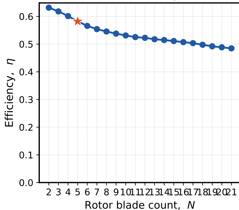
(c) efficiency
