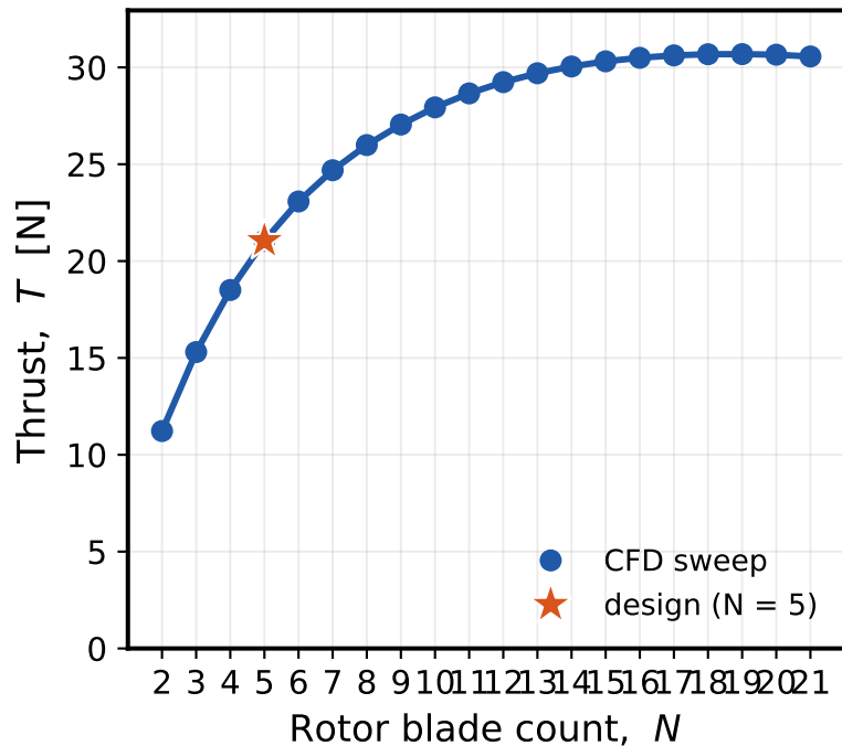
(a) thrust
