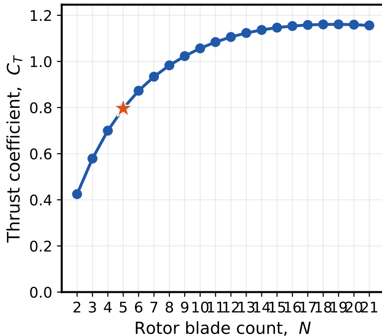
(b) thrust coefficient
