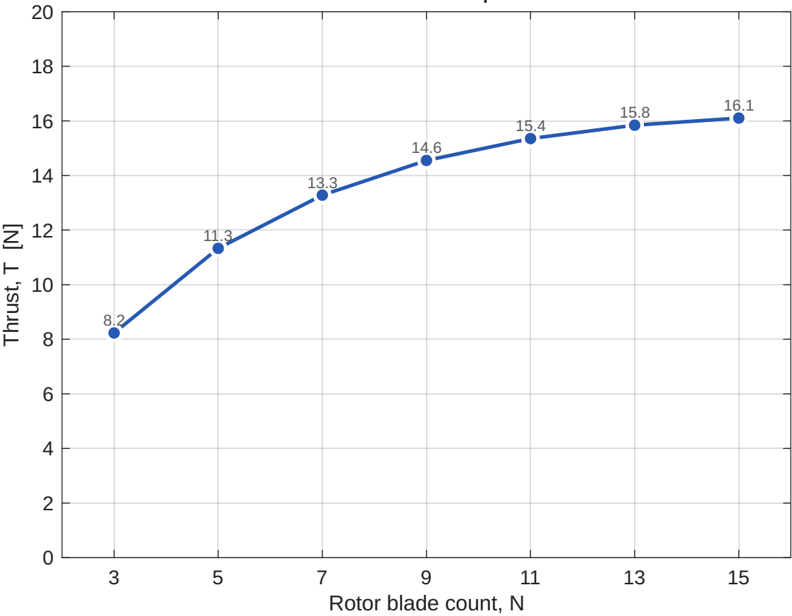
Propeller thrust vs blade count ( V_f = 20 m/s, RPM = 8191)
