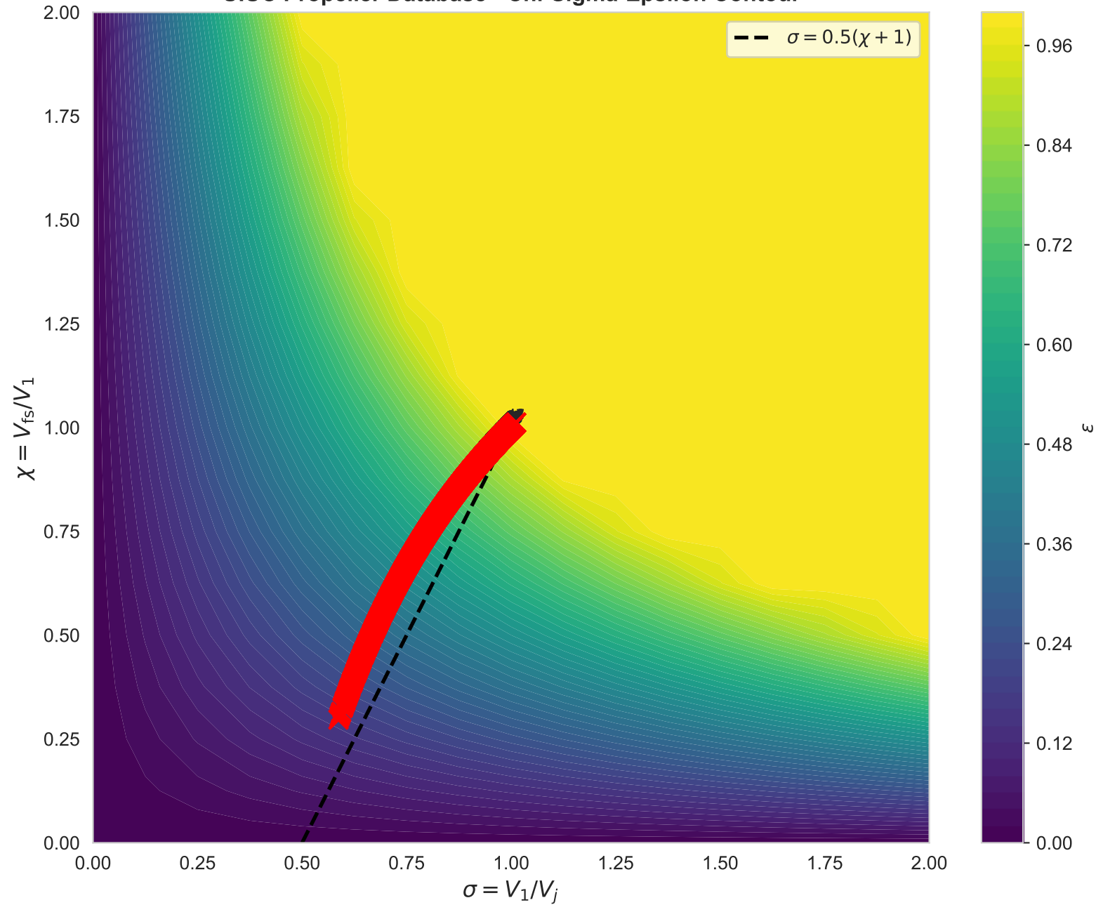
UIUC Propeller Database - Chi-Sigma-Epsilon Contour
