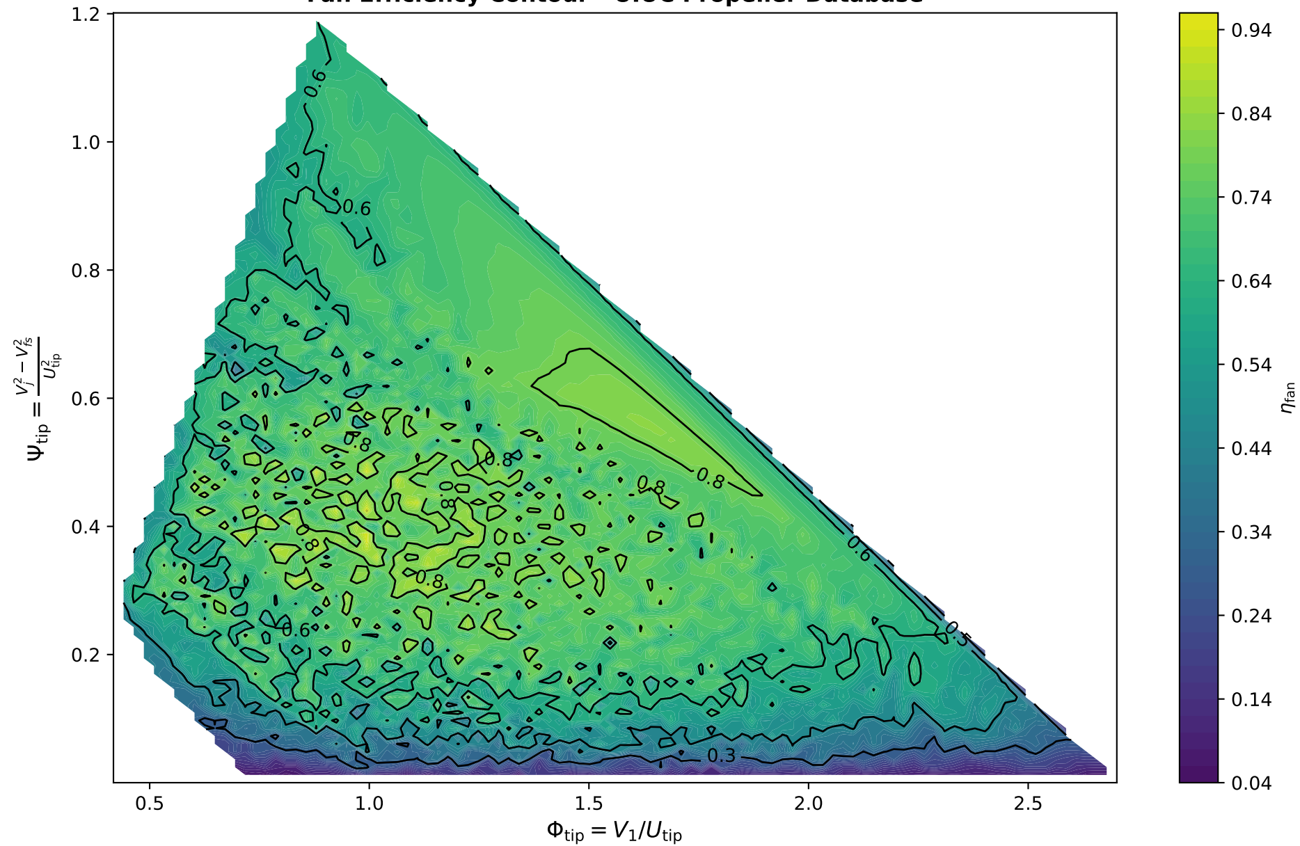
Fan Efficiency Contour - UIUC Propeller Database
